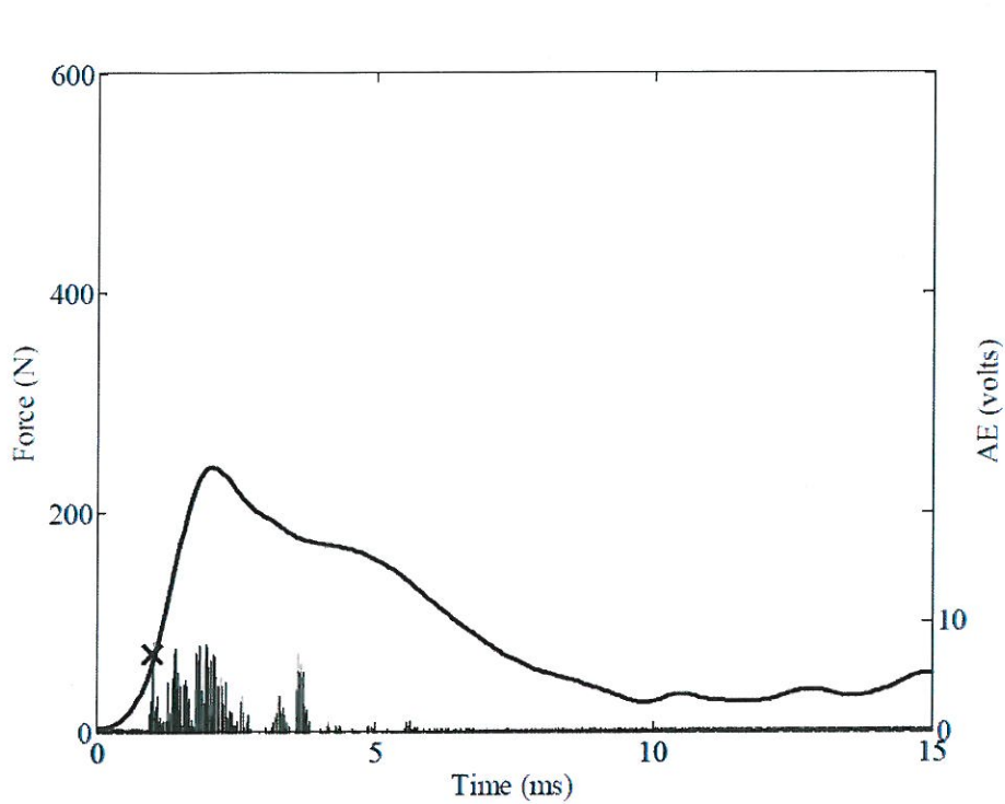
Figure 32: Force and AE response for subject 43.
