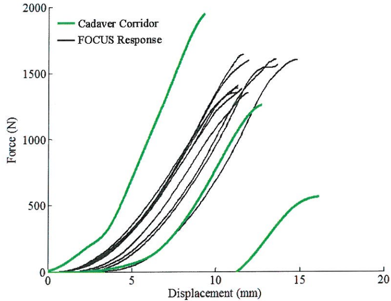
Figure 38: Zygoma response during FOCUS and cadaver testing.
