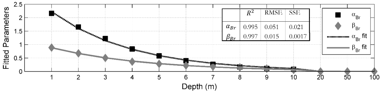
Figure 15. The calculated values of \alpha_{Br} and \beta_{Br} of function (3.11) are plotted with squares and diamonds, respectively. The two lines correspond to the fitted models of the two parameters, and the different statistical measures of goodness-of-fit are tabulated.
