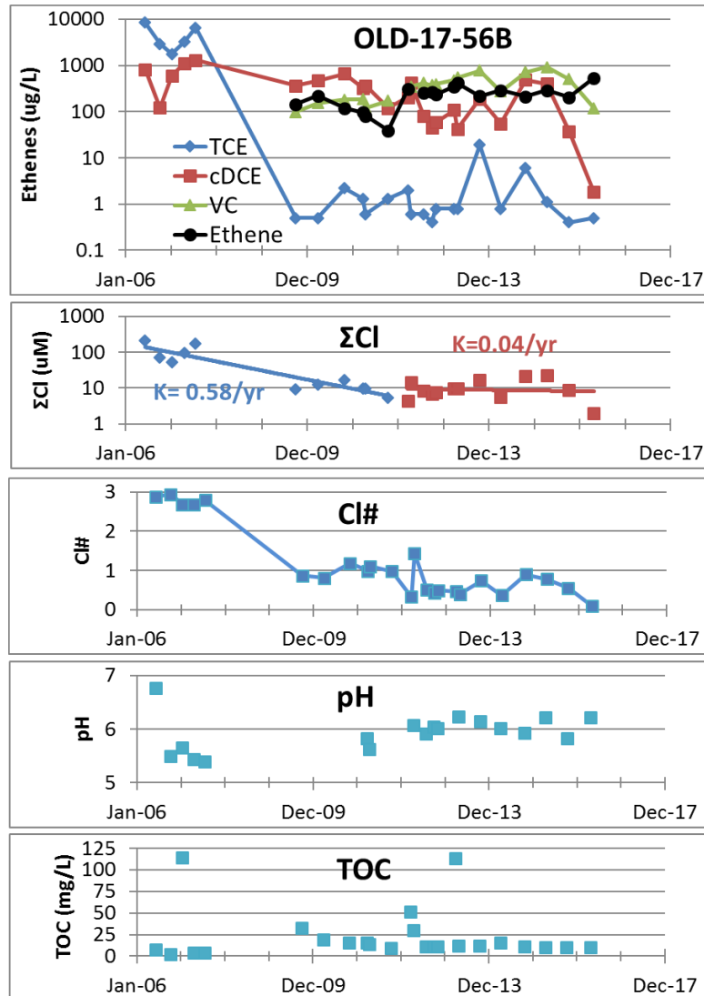
Figure 6. Variation in TCE, cDCE, VC, Ethene, \Sigma\text{Cl} , \text{Cl}\# , pH and TOC versus Time in OLD-17-56B.
