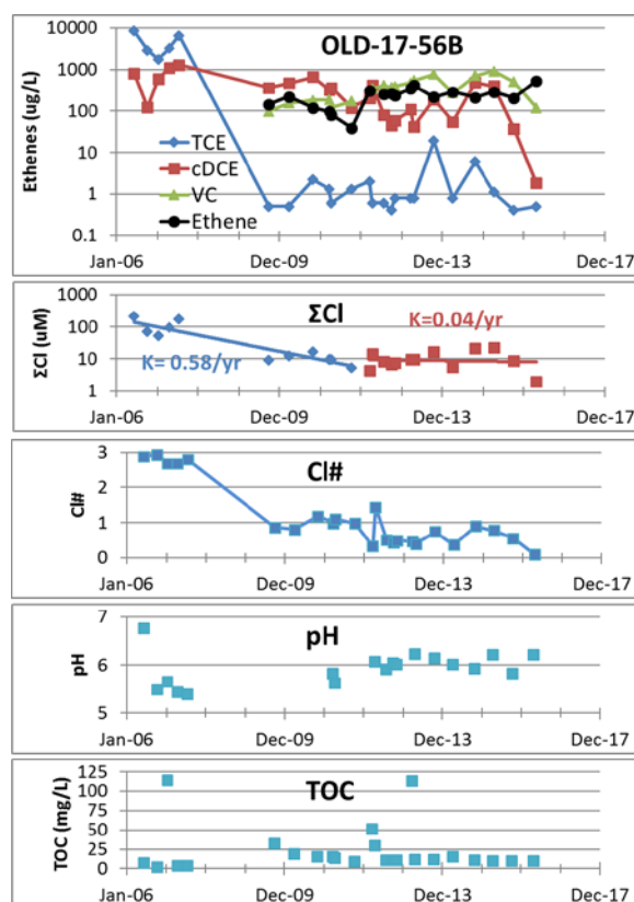
Figure B-7. Variation in TCE, cDCE, VC, Ethene, \Sigma\text{Cl} , Cl#, pH and TOC versus Time in OLD-17-56B.
