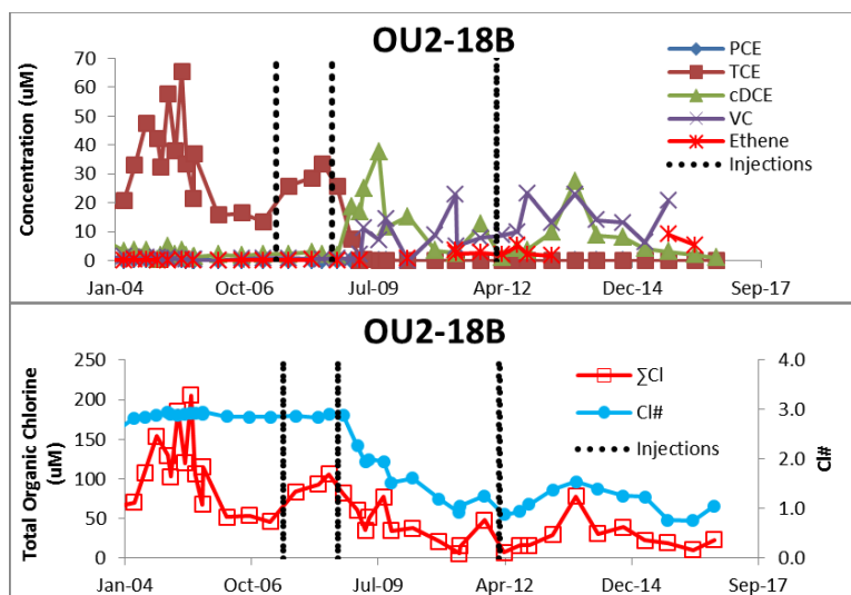
Figure C-8. Variation in TCE, cDCE, VC, Ethene, \Sigma\text{Cl} , and \text{Cl}\# versus Time in OU2-18B.
