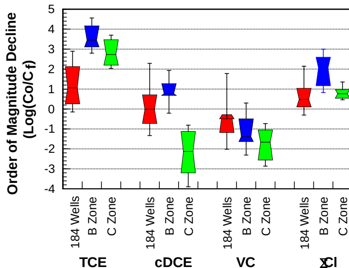
Figure B-11. Order of Magnitude (OoM) Decline in TCE, cDCE, VC and \Sigma Cl for 184 Wells Reported by Tillotson and Borden (2017) and for SA17 B and C Zone Monitoring Wells.
