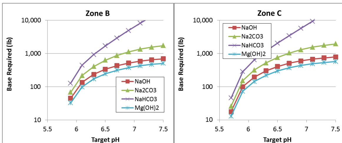
Figure B-13. Required base addition for 2012 SA17 zones B and C for different target pH values.
