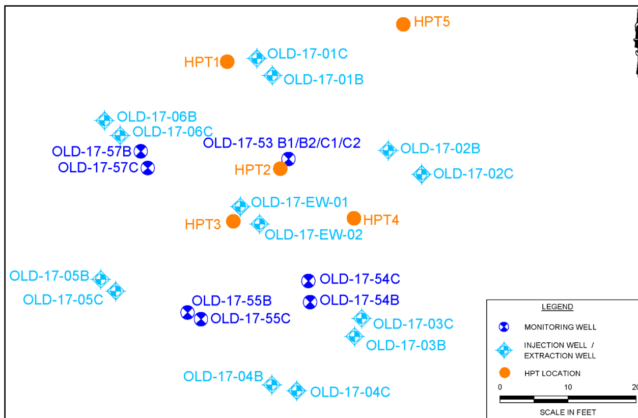
Figure B-2. Location of HPT Profiles, Soil Borings, Injection and Monitor Wells near SA17 Bioremediation Project.
