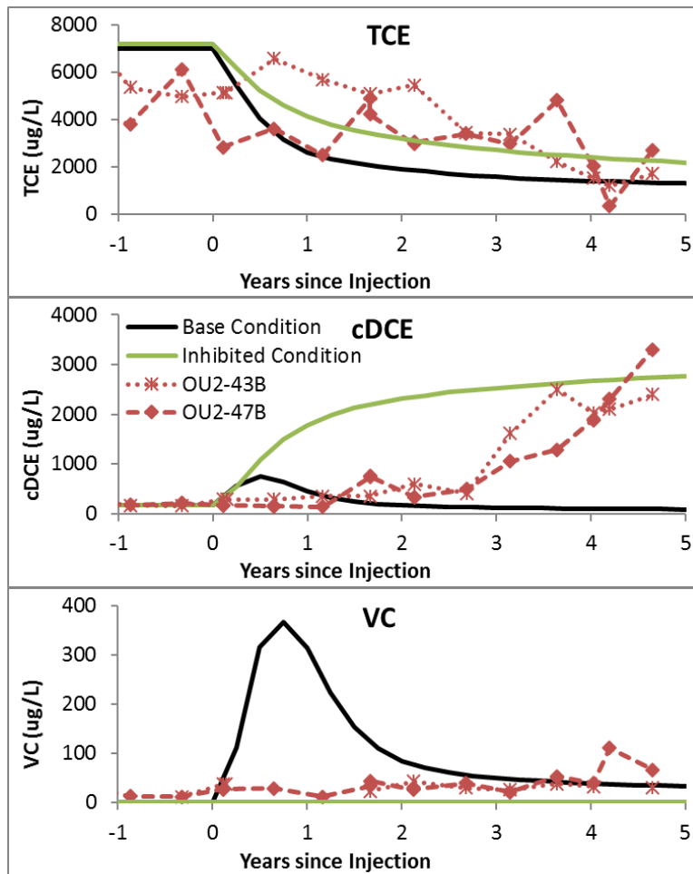
Figure C-17. Comparison of measured and simulated TCE, cDCE, and VC concentrations in the northern study area.
