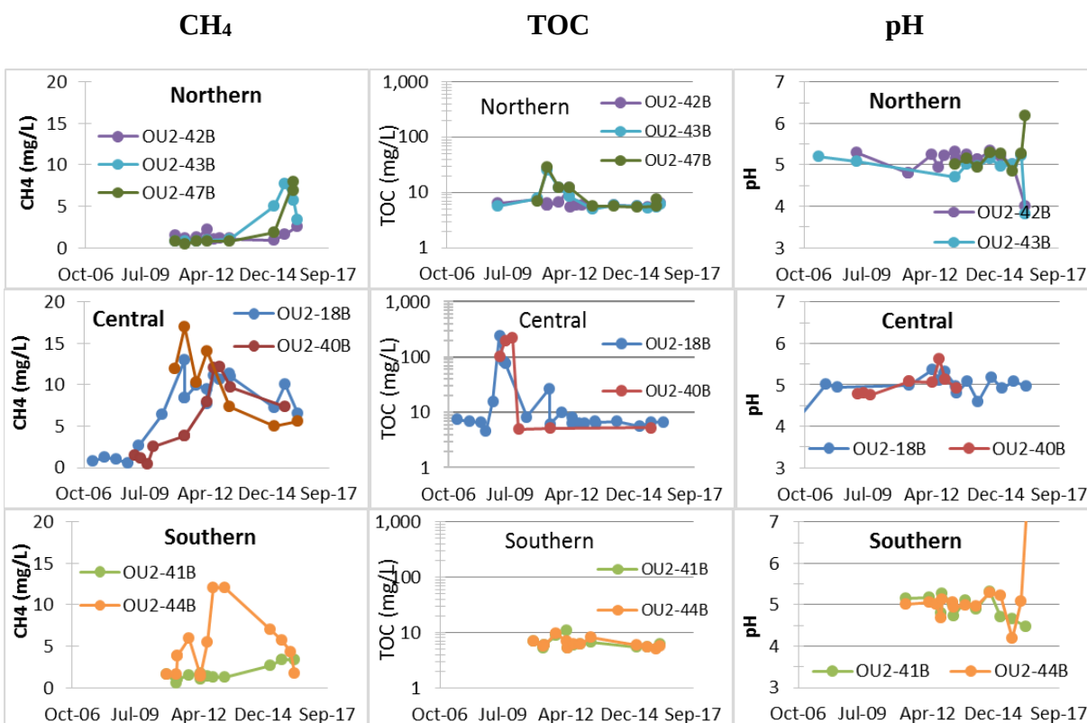
Figure 12. \text{CH}_4 , TOC, and pH in Monitor Wells Downgradient of the Northern, Central, and Southern Portions of the EVO PRB.
