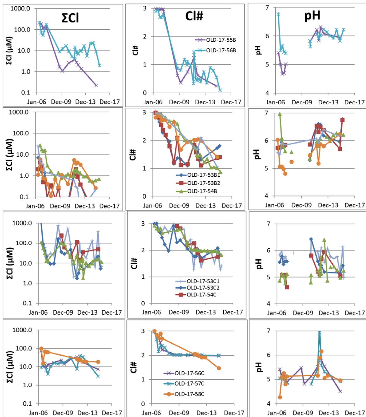
Figure B-8. Variation in ΣCl, Cl# and pH in Zone B and C Monitor Wells.
