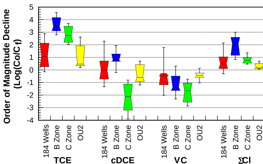
Figure 20. Order of Magnitude (OoM) Decline in TCE, cDCE, VC, and \Sigma Cl for 184 Wells (Tillotson and Borden, 2017), SA17 B and C Zones Monitoring Wells, and OU2 Monitoring Wells.
