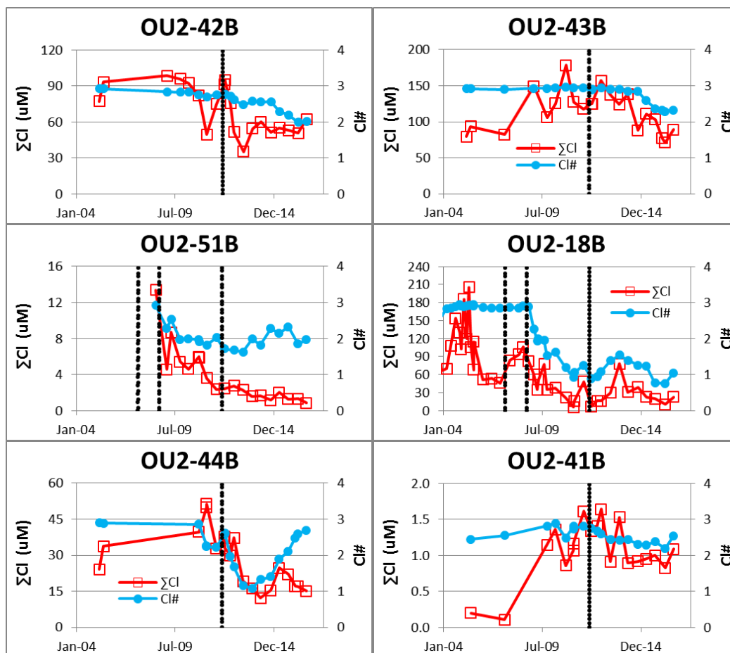
Figure C-9. Variation in \Sigma\text{Cl} and \text{Cl}\# in Monitor Wells Downgradient of the Northern (OU2-42B and OU2-43B), Central (OU2-51B and OU2-18B), and Southern (OU2-44B and OU2-41B) Portions of the EVO PRB.
