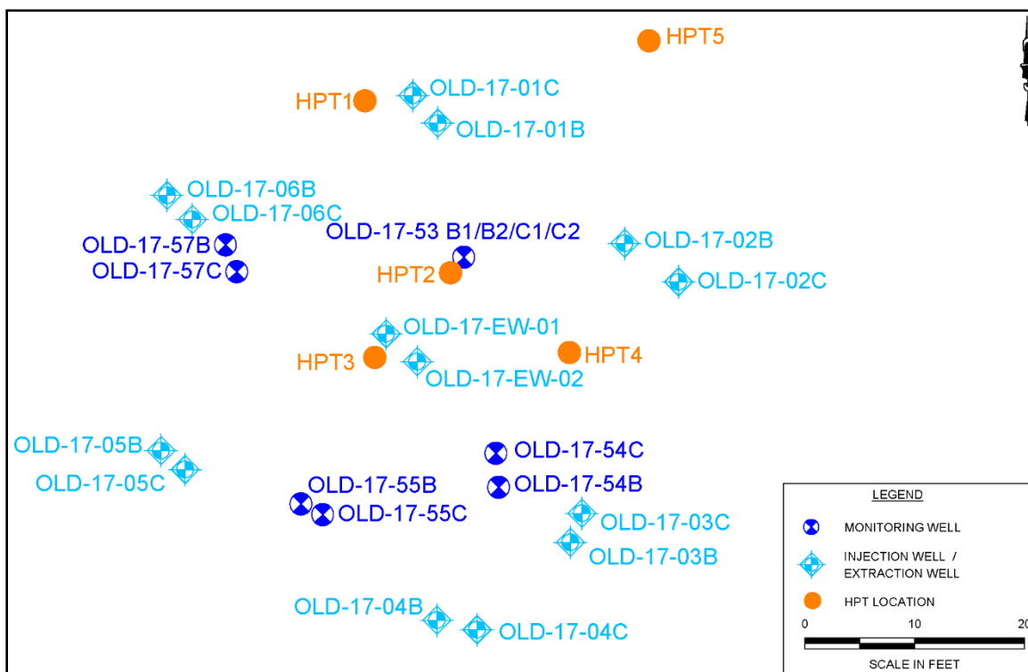
Figure 4. Injection and Monitor Wells in the Vicinity of SA17 Bioremediation Project.
