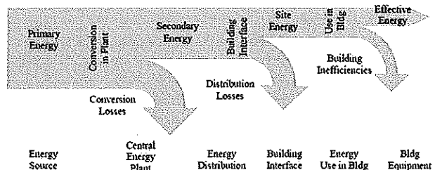
Figure 9 Energy supply chain from primary energy to its use inside a building.
