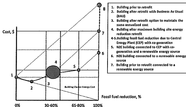
Figure 12 Building fossil fuel reduction optimization process.
