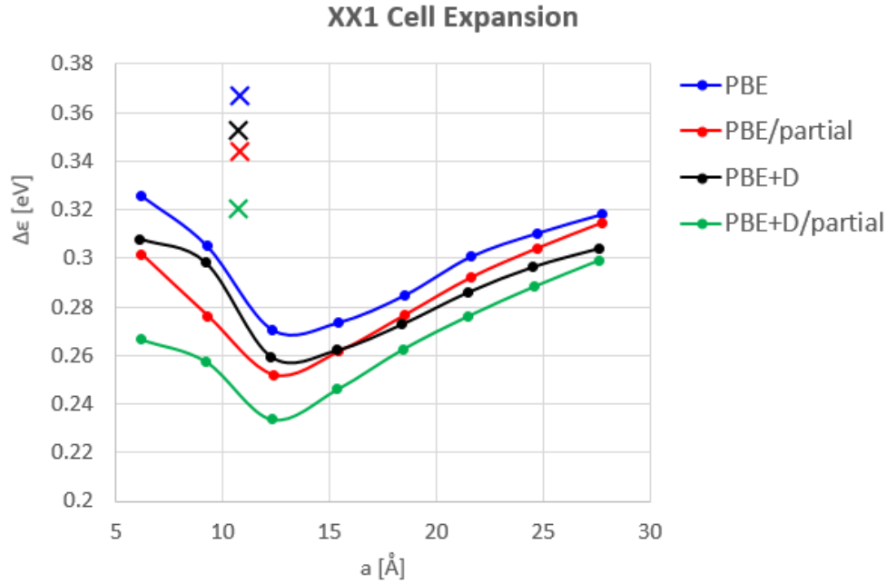
Fig. 9 Highest occupied defect level relative to bulk valence band maximum ( \Delta\epsilon ) in eV for the hh divacancy defect in 4H-SiC as a function of the cell parameter a in Å while c is kept at unit cell value, PBE with and without D, and full and partial relaxation. Data points marked x are obtained with the 341-cell expansion, and values for a are averaged.
