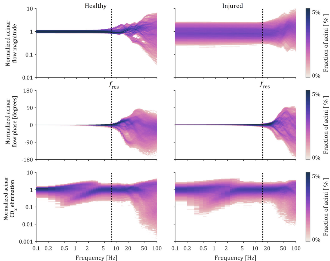
Fig. 8. Simulation representing model predictions for eupneic ventilation vs. oscillatory frequency. Horizontal axes are aligned, dashed black lines represent the resonant frequency ( f_{\text{res}} : elastic and inertial components of impedance equal and opposite). Acinar flow magnitude, flow phase, and \text{CO}_2 elimination are normalized as described in the text.
