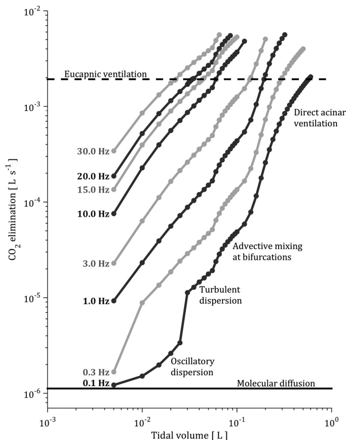
Fig. 4. Simulation results for \dot{V}_{\text{tot}}\text{CO}_2 as a function of V_T and f . Solid black horizontal line represent the lower bound of total \text{CO}_2 elimination due solely to molecular diffusion (i.e., zero-flow conditions), while the dashed horizontal line represents total \text{CO}_2 elimination to achieve eucapnia for a 25 kg dog. Text labels indicate dominant gas transport mechanism during 0.1 Hz oscillation.
