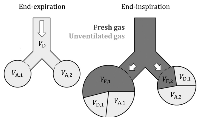
Fig. 3. Direct acinar ventilation is modeled by assuming complete mixing within each n th terminal acinus of inspired fresh gas ( V_{F,n} ), inspired dead space gas ( V_{D,n} ), and residual volume ( V_{A,n} ). The concept of “personal dead space” is used to distribute the total dead space ( V_D ) throughout all acini in proportion to the magnitude of the ventilation distribution (13).
