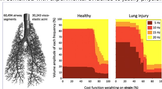
Figure 1: Computational model of porcine lung (left panel). Optimal volume amplitudes at each frequency are shown for varying cost function emphasis on strain vs. strain rate, in simulated healthy conditions (center panel) and heterogeneous lung injury (right panel).
