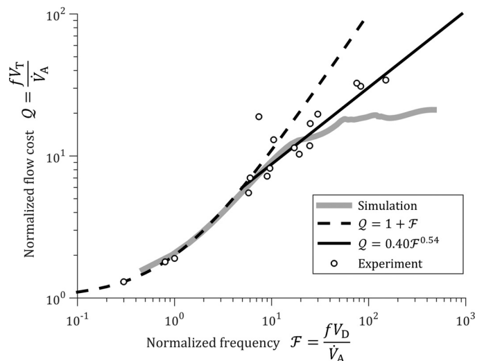
Fig. 6. Comparison between simulation results and experimental data of Venegas et al. (47). The axes are dimensionless variables of frequency ( F ) and flow ( Q ). The black lines correspond to theoretical predictions of low-frequency gas exchange (dashed) and regression to experimental HFOV data (solid). The gray line represents the simulations results interpolated at eucapnic conditions.
