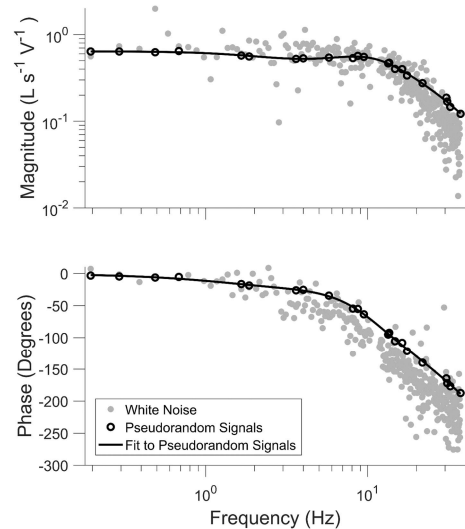
Figure 1 Frequency response of PSOL valve driven with white noise (gray symbols) and pseudorandom signal (black symbols) inputs, along with corresponding fit of Equation 1 to pseudorandom data (solid lines).
