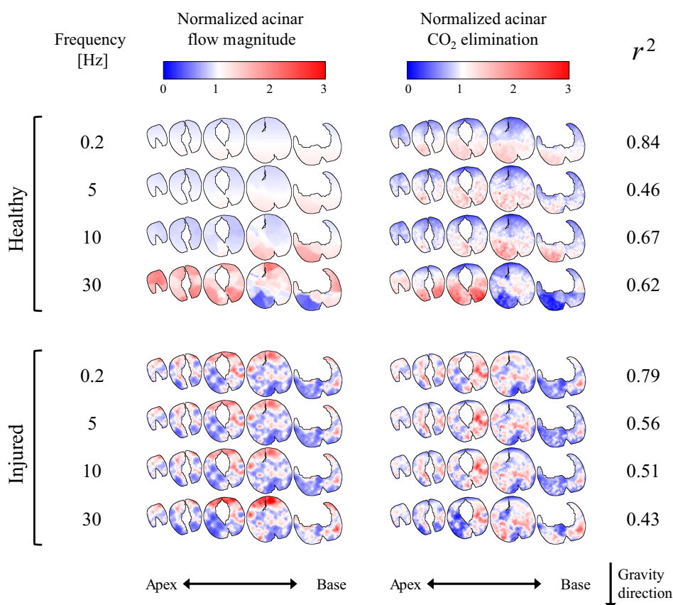
Fig. 7. Transverse cross sections of simulated regional acinar flow magnitude (left) and CO 2 elimination (right) at selected oscillatory frequencies, for healthy (top) and injured (bottom) conditions, spatially interpolated between acinar elements for visualization. Coefficients of determination ( r^2 ) between acinar flow magnitude and CO 2 elimination are shown at the far right.
