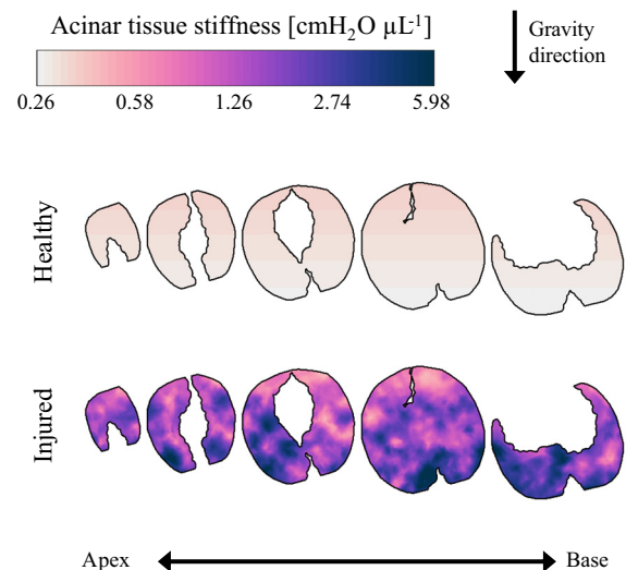
Fig. 2. Transverse cross sections of simulated regional acinar tissue stiffness for healthy (upper) and injured (lower) conditions, spatially interpolated between acinar elements for visualization.
