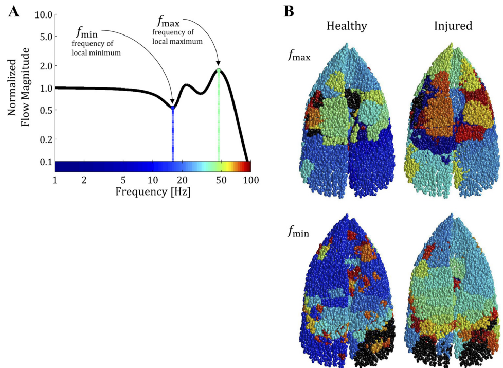
Fig. 9. A: frequencies of maximum and minimum normalized flow magnitude, shown for clarity in the context of a single acinus. B: frequencies of maximum (top) and minimum (bottom) normalized flow magnitude, represented spatially for every acinus, using consistent coloring according to the scale provided in A. Acinar flow magnitude is normalized to the uniform distribution (unity corresponds to tracheal magnitude divided by total number of acini). Acini that do not exhibit a local minimum or maximum within the range of frequencies simulated are shown in black. The gravitational vector points out of the page, toward the reader.
