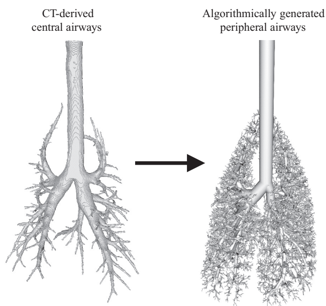
Fig. 1. Central airways of a canine lung as segmented from an X-ray computed tomographic scan in a supine dog (left) and resulting anatomically based 3-dimensional airway network (right) generated using a space-filling algorithm (38, 39).
