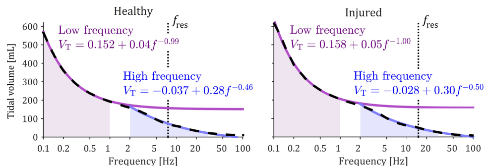
Fig. 5. Simulation results representing model predictions for eucapnic ventilation at various single frequencies of oscillation (dashed black lines). Dotted vertical black lines represent the resonant frequency ( f_{\text{res}} : elastic and inertial components of impedance equal and opposite). Model predictions of tidal volume required for eucapnic ventilation derived from power-law regressions over low frequencies (purple: 0.1 \leq f \leq 1 \text{ Hz} ) and high frequencies (blue: 2 \leq f \leq 30 \text{ Hz} ).
