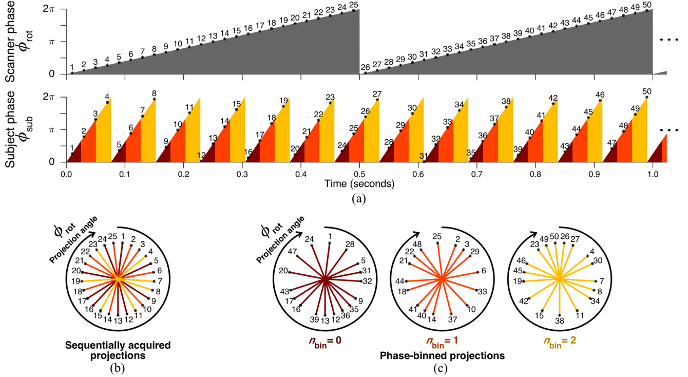
Fig. 1. Illustration of FSCT concept for arbitrarily selected parameters. (a) Scanner phase \phi_{\text{rot}} as a function of time for a 2.0 Hz rotation frequency, with 25 projections acquired per rotation as indicated by numbered asterisks. Projections are numbered according to chronological order of acquisition. Subject phase \phi_{\text{sub}} as a function of time for a 13.13 Hz periodic motion cycle. Subject phase is labeled according to 3 equally sized bins, indicated by color (red, orange, yellow). (b) Standard CT reconstruction is performed on sequentially acquired projections, averaging together variable subject motion phase acquired throughout one scanner rotation. (c) FSCT reconstruction is performed on phase-binned subsets of projections, each containing a limited range of subject phase.
