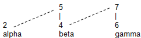
Figure 9: Constituent Parsing Example; Initial Derived Constituent Structure
