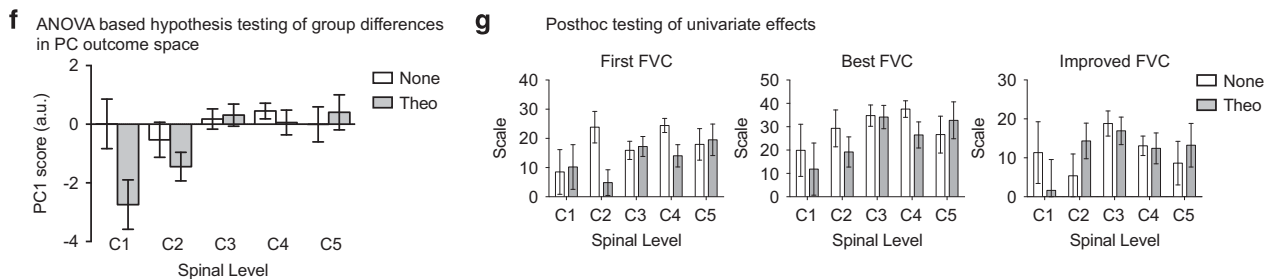
Figure 1 Statistical analysis workflow. (a) Data distribution of each clinically relevant outcome was assessed to determine the type of statistical tests to use. (b) Correlation matrix of all outcomes used to perform (c) nonlinear principal component analysis (NL-PCA) to identify three principal components (PC) based on both having eigenvalues greater than 1 whose (d) multivariate outcomes also had face validity to the clinicians who collected the data. (e) Composite PC scores from each multivariate outcome was assigned to each patient and used to map each subject into a three-dimensional space based on their syndromic outcomes generated with NL-PCA. Workflows a–e were all conducted blinded to treatment condition. (f) Hypothesis testing was performed on multivariate outcomes (PC1–PC3) for interactions between type of treatment (group 1 vs group 2) and SCI spinal level on the multivariate space. (g) Individual outcomes tested with the same hypothesis using univariate statistics, demonstrating that only the multivariate outcomes are sufficiently powered for hypothesis testing, whereas individual outcomes separately cannot reliably test these hypotheses.
