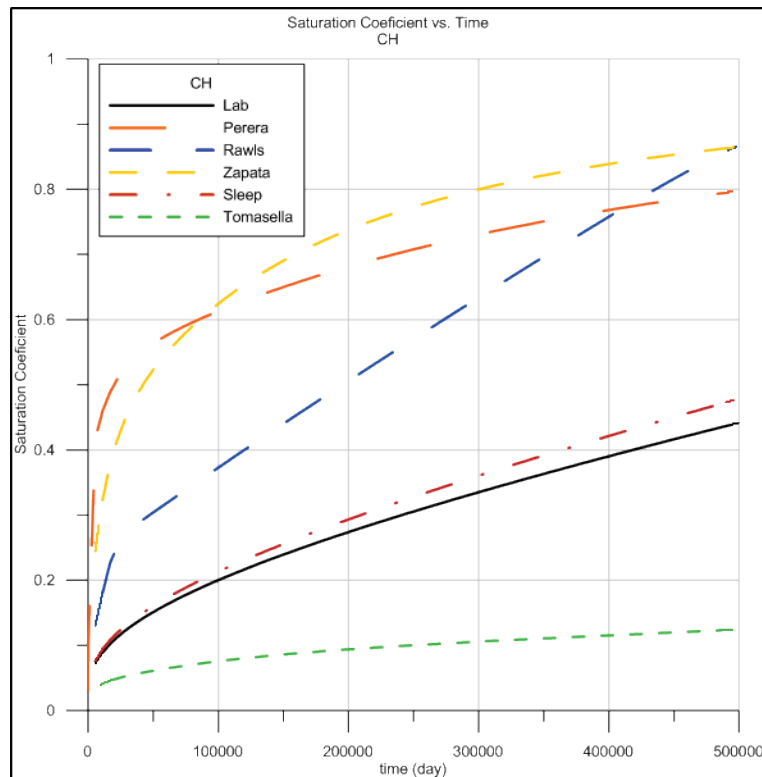
Figure 18. Saturation versus time for the CH material.
