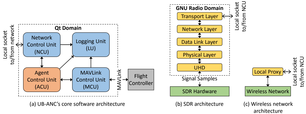
Figure 11: High-level software architecture diagram. (a) UB-ANC's core software architecture with its interface to the network. (b) SDR architecture with its interface to the Network Control Unit. (c) Standard wireless network architecture with its interface to the Network Control Unit.
