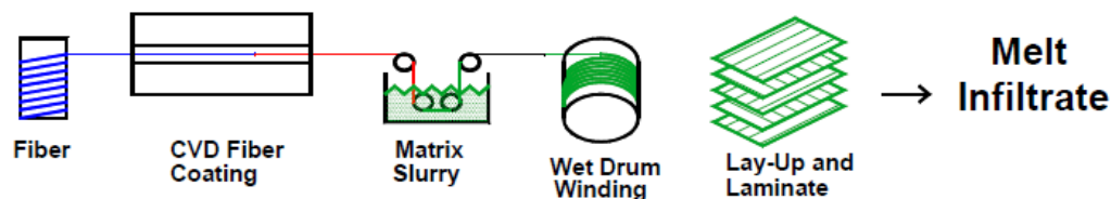
Figure 1. A simple schematic of the manufacturing process used to manufacture the CMC panel used in this study
