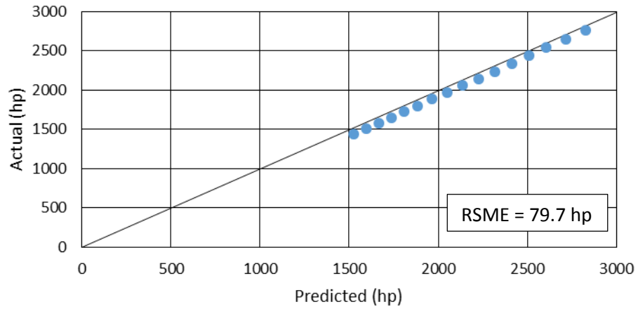
Figure 25. UH-60L Hover Power Required Actual vs Predicted at 4000 ft, 95 °F
