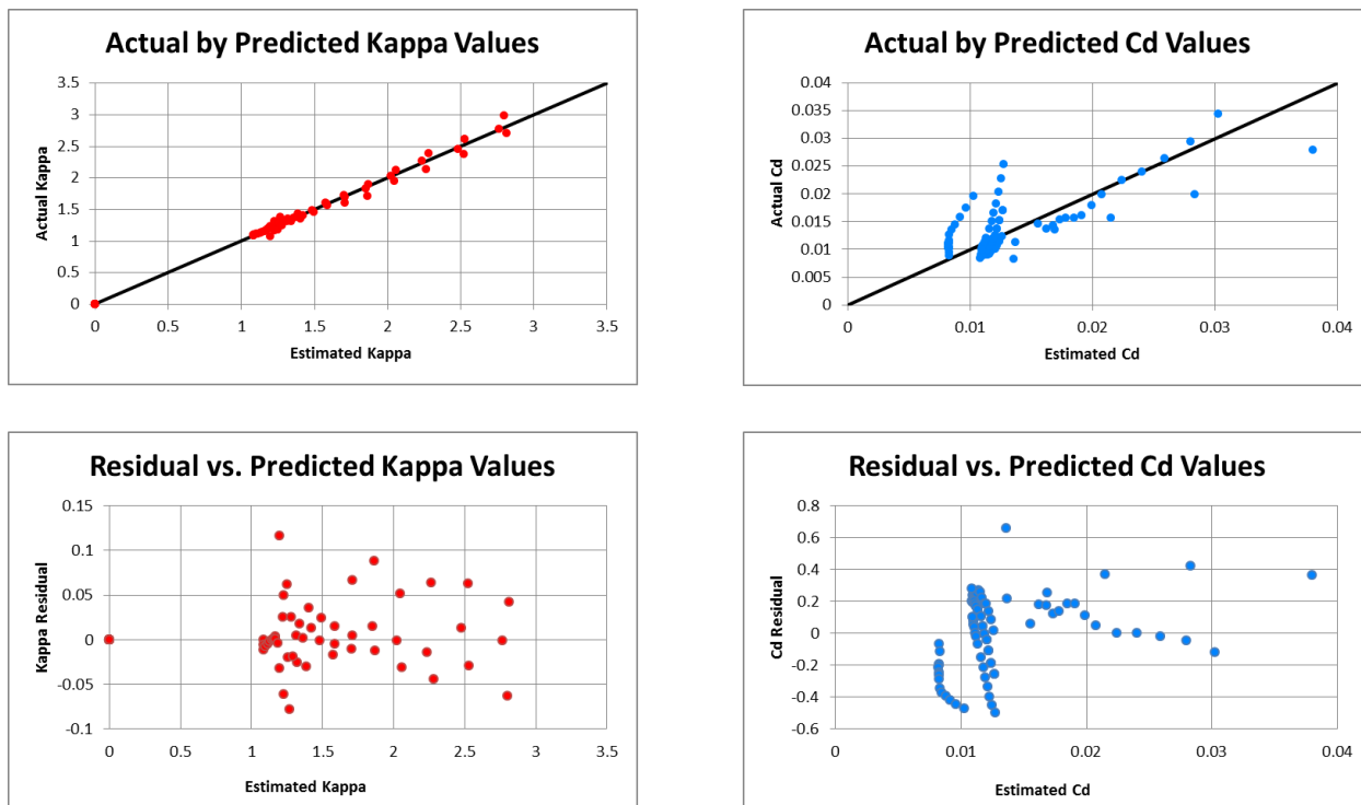
Figure 4-20: Example of results for a good fit (Kappa values) and poor fit (Cd values) on the actual by predicted and residual by predicted plots
