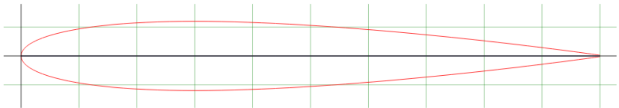
Figure 42: NACA0012 Airfoil
