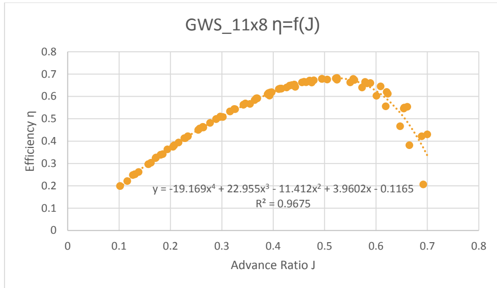
Figure 54: Regression of Propeller Efficiency
