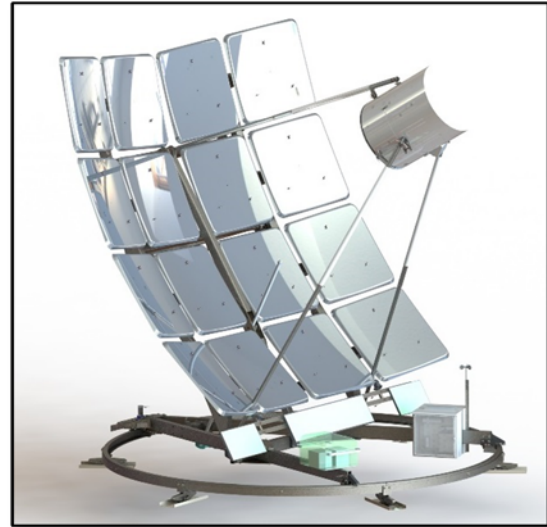
Figure 11: SPSWH Helia Enhancement Prototype II
