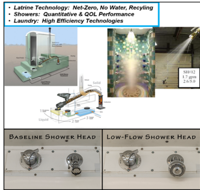
Figure 57: Water Demand Reduction Concept
