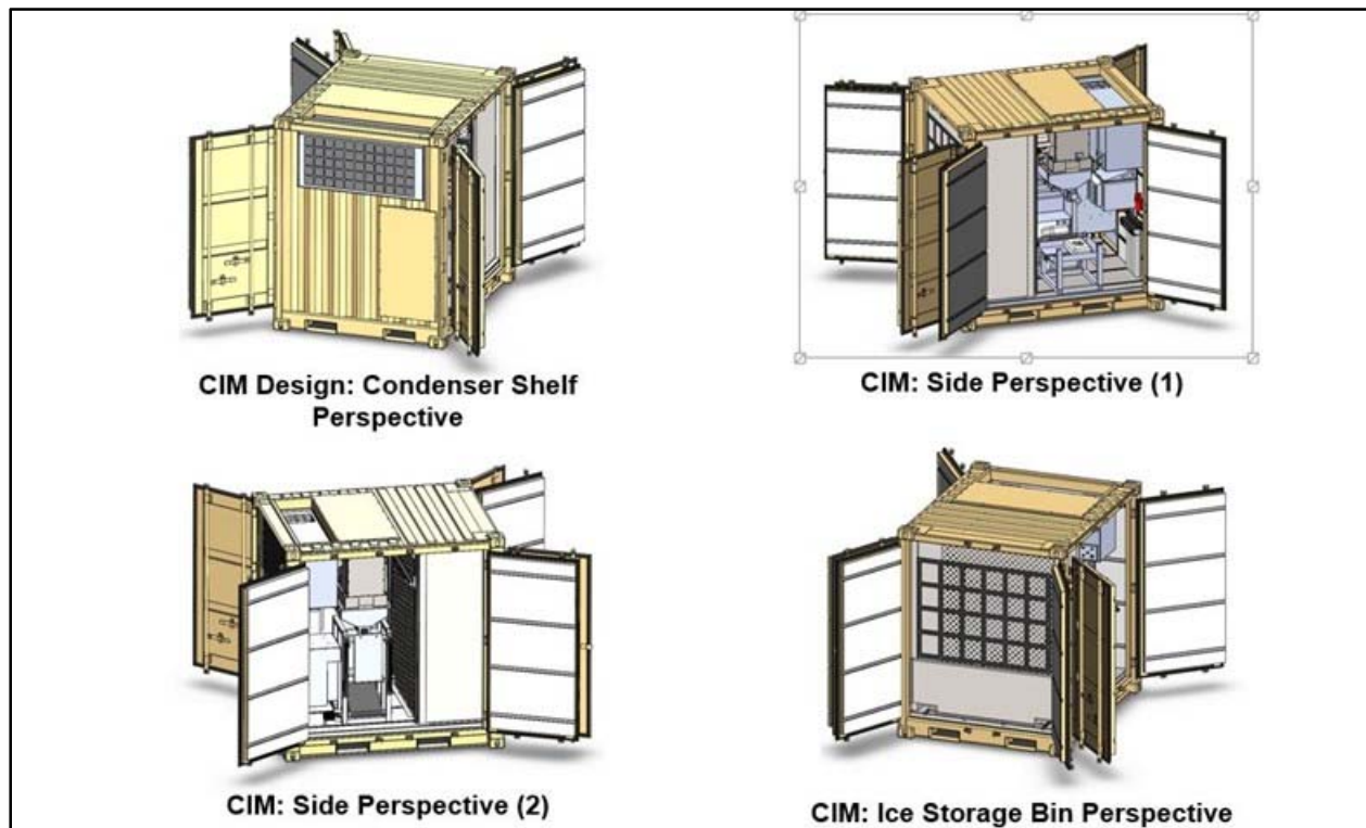
Figure 76: Rocky Research TRICON CIMS
