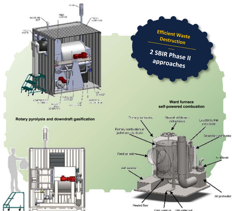
Figure 59: Solid Waste Destruction System
