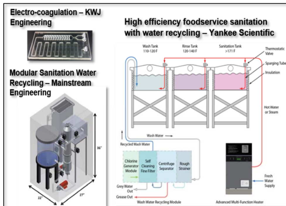
Figure 48: Water Conservation Technology
