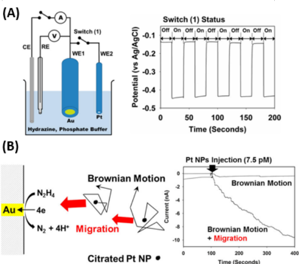
Figure 4: (A) Schematic depicting the effective nanoparticle collision experiments where a Pt nanoelectrode was used as a model nanoparticle and connected by a switch to a Au UME and the magnitude of the OCP change upon switching could be repeatedly measured. (B) Effect of migration on the collision frequency of nanoparticles to a Au UME where the collision frequency is observed to be much higher than predicated for diffusion alone.
