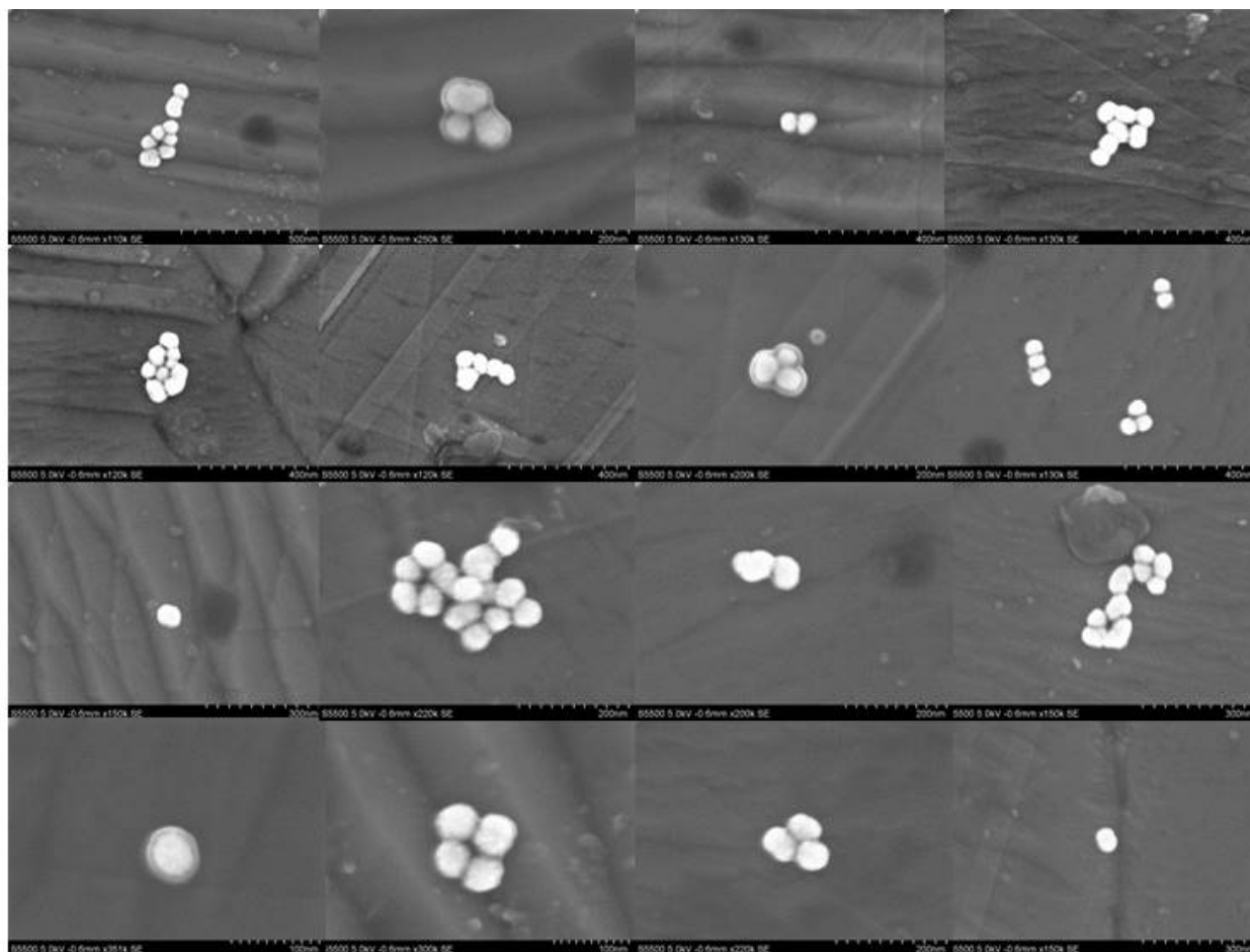
Figure 4. SEMs of Pt NPs that adsorbed on stainless steel foil from solution of 10 mM \text{N}_2\text{H}_4 + 50 mM SPB, pH 7.8 over the course of one hour at 1.1 pM Pt NP concentration.
