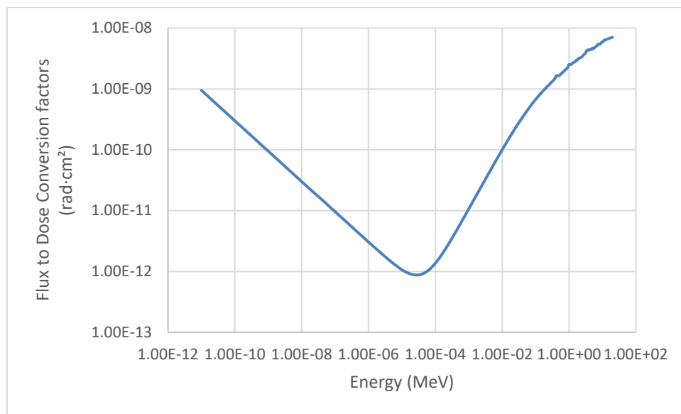
Figure 2.5 Response function for neutron radiation
