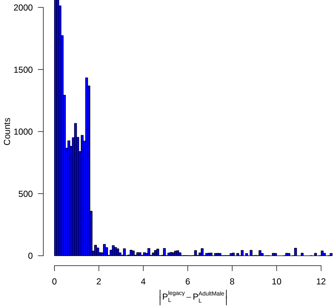
Figure 3.15: Histogram, magnitude of difference between probability of lethality given by legacy table ( P_L^{\text{legacy}} ) and probability of lethality calculated by HENRE for adult male ( P_L^{\text{AdultMale}} ), protection factor 7
