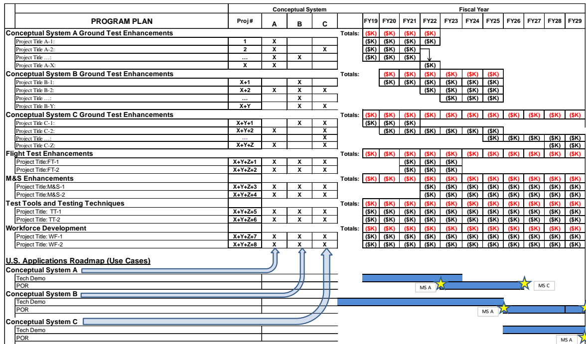
Fig. 3 Plan Roadmap.
