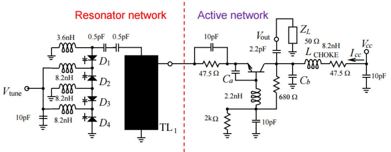
Figure 4 Tunable SiGe BJT VCO
