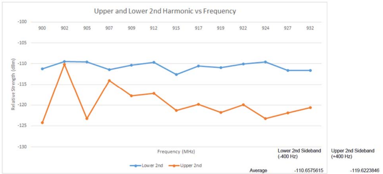
Figure 37: Asymmetric sidebands of acoustically stimulated vibrations.
