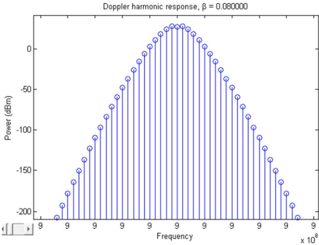
Figure 32: Expected roll off using Doppler model. This used the amplitude of the vibrations recorded by the LDV at corresponding mechanical vibration frequencies.
