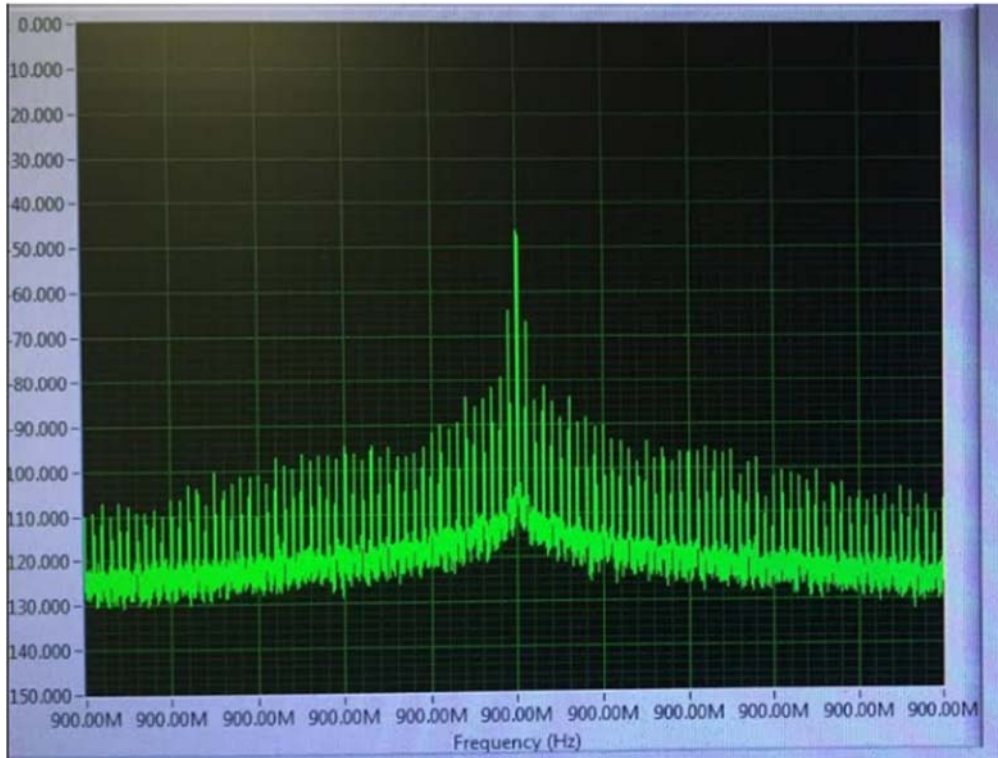
Figure 31: Signal “reflected” from vibrating antenna with 10 kHz span.
