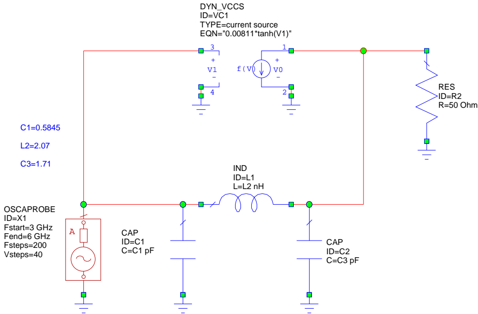
Figure 14: Schematic of the simplified oscillator model.
