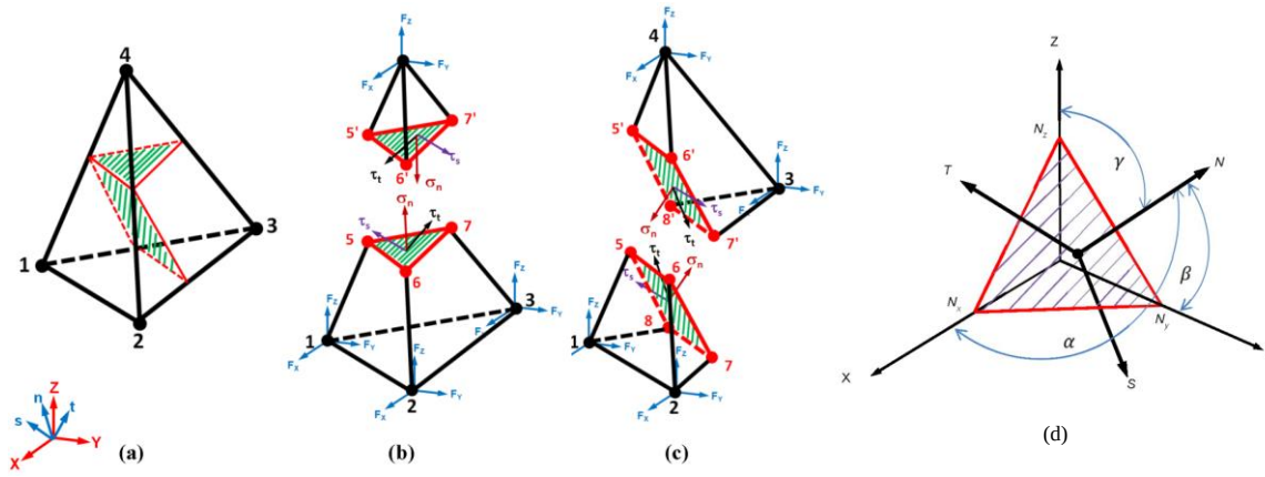
Figure 5: Element illustration for (a) a regular 4-node tetrahedron element with two possible cut configurations by a crack plane, (b) the A-FE with tetrahedron-wedge configuration, (c) the A-FE with wedge-wedge configuration, (d) definition of local coordinates for the crack plane.
