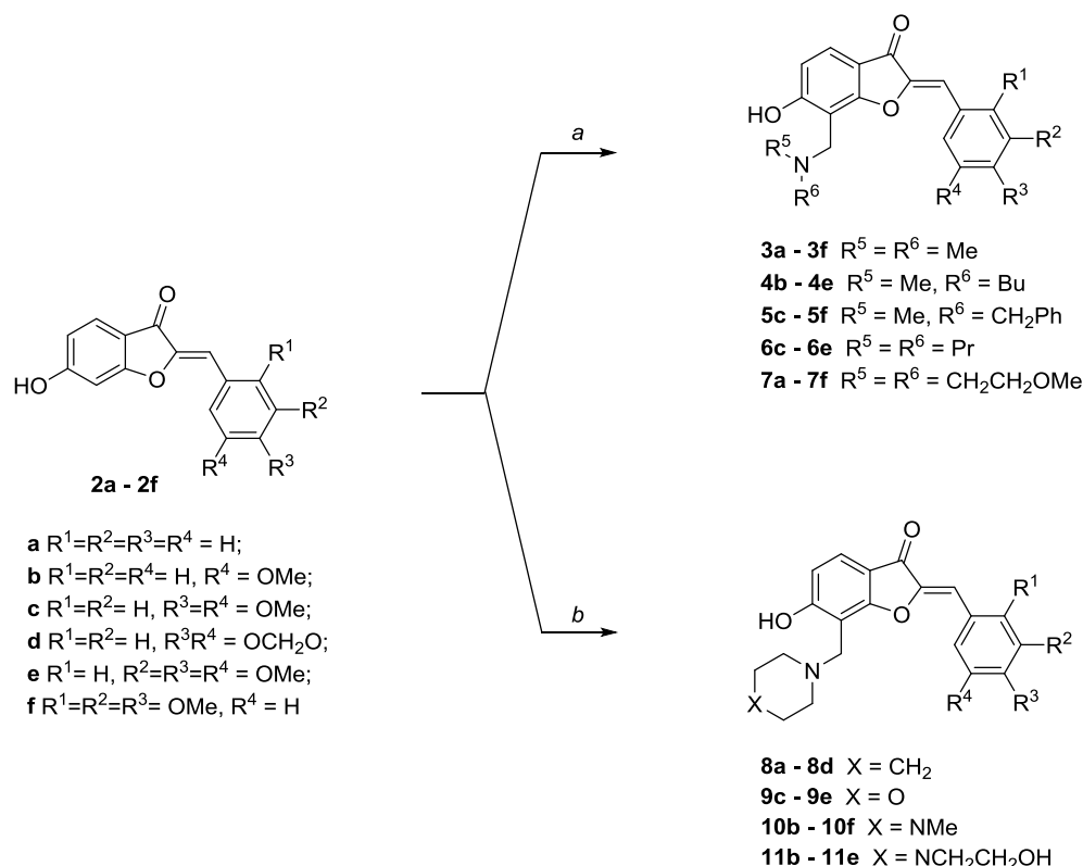
Scheme 1. Synthesis of Mannich bases of 6-hydroxyaurones 3-11 . Reagents and conditions: a) CH_2(NR^5R^6)_2 , i -PrOH, 80°C, 4-8 h; b) CH_2(NC_4H_8X)_2 , i -PrOH, 80°C, 4-6 h
