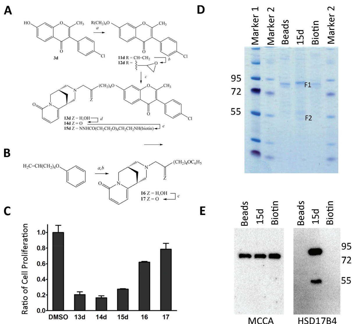
Fig. 3 A. Synthesis of a biotinylated cytisine-linked isoflavone 15d . Reagent legend: a, K 2 CO 3 , 6-bromo-1-hexene (yield: 81%); b, MCPBA (yield: 76%); c, cytisine, EtOH, 90 °C, pressure tube (yield: 96%); d, Dess–Martin reagent (yield: 81%); e, PEG hydrazide, CeCl 3 (yield: 24%). B. Reagent legend: a, MCPBA (yield: 81%); b, cytisine, EtOH, 90 °C, pressure tube (yield: 98%); c, Dess–Martin reagent (yield: 57%). Specific yields for individual isoflavonoids are given in the ESI.† C. Effects of isoflavonoids 13–17 on the proliferation of PC-3 cells. D. Purification of binding proteins of isoflavonoids. E. Validation of potential targets using western blotting.
