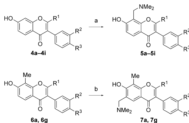
Scheme 1. Regioselective modification of 7-hydroxyisoflavones 4 and 7-hydroxy-8-methylisoflavones 6 . Reagents and conditions: a) CH 2 (NMe) 2 , iPrOH, 80 °C, 2–4 h, 68–91%; b) CH 2 (NMe) 2 , dioxane, 100 °C, 16 h, 72–99%.
