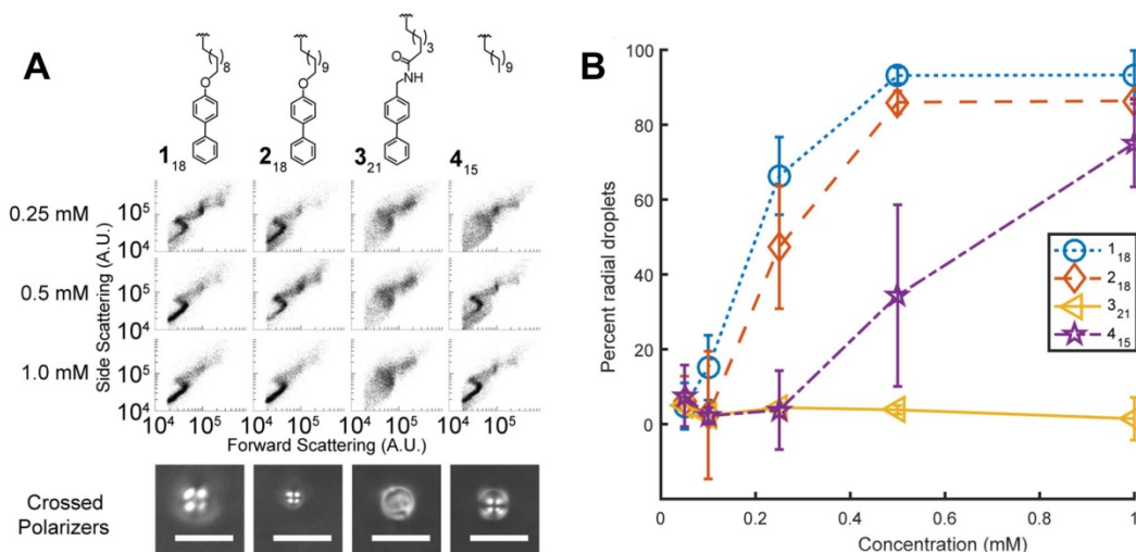
Figure 11 (A) Scatter plots generated from flow cytometry of LC droplets decorated with polymers 1-4 (Fig. 1-4) and crossed polarized microscopy images. (B) The percentage of radial droplets generated as a function of the polymer and polymer concentration, calculated from the scatter plots.
