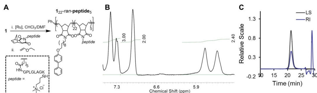
Figure 43 Polymerization and characterization of 1 22 -ran-peptide 5 . (A) Polymerization of monomers 1 and peptide to afford random copolymer 1 22 -ran-peptide 5 . (B) 1 H-NMR of 1 22 -ran-peptide 5 to confirm complete polymerization ( 1 : peptide :I = 20:10:1). Monomer ratios are estimated from the relative integration of biphenyl proton resonances and polymer backbone olefin protons. (C) SEC-MALS data of copolymer 1 22 -ran-peptide 5 ; Mn = 15,800 g/mol, Mw/Mn = 1.015, (dn/dc = 0.179).
