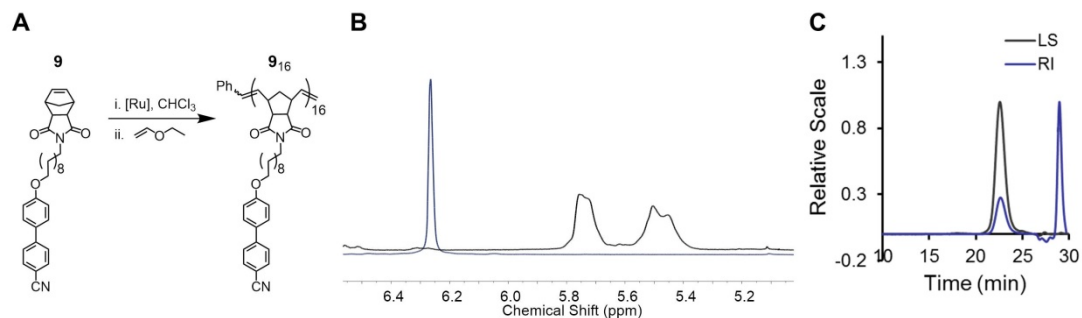
Figure 30 P Polymerization and characterization of 9 16 . (A) Polymerization of monomer 9 to afford homopolymer 9 16 . (B) 1H-NMR of 9 to confirm complete polymerization (M:I = 20:1). Spectra of the monomer and polymer depict olefin resonances and are shown in blue and black, respectively. (C) SEC-MALS data of polymer 9 16 ; Mn = 8,077 g/mol, Mw/Mn = 1.017, (dn/dc = 0.179).
