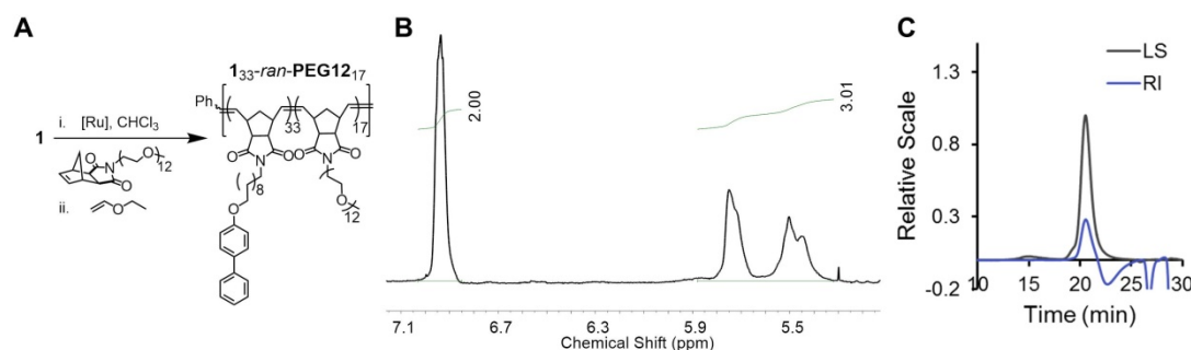
Figure 42 Polymerization and characterization of 1 33 -ran-PEG12 17 . (A) Polymerization of monomers 1 and PEG12 to afford random copolymer 1 33 -ran-PEG12 17 . (B) 1 H-NMR of 1 33 -ran-PEG12 17 to confirm complete polymerization ( 1 : PEG12 :I = 32:8:1). Monomer ratios are estimated from the relative integration of biphenyl proton resonances and polymer backbone olefin protons. (C) SEC-MALS data of copolymer 1 33 -ran-PEG12 17 ; Mn = 27,090 g/mol, Mw/Mn = 1.019, (dn/dc = 0.1375).
