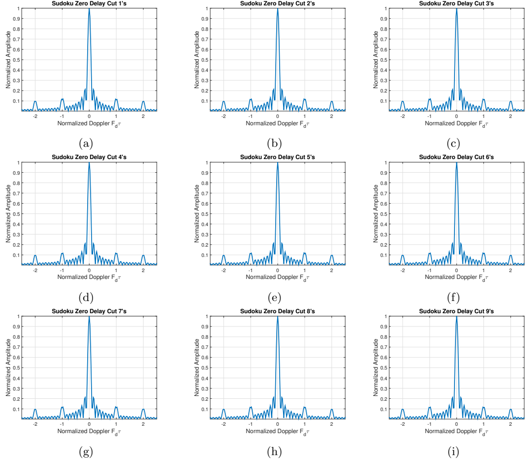
Figure 13: The zero delay cuts for the individual numbers of the previously described Sudoku puzzle solution. (a) number 1s, (b) number 2s, (c) number 3s (d) number 4s, (e) number 5s, (f) number 6s, (g) number 7s, (h) number 8s, (i) number 9s.
