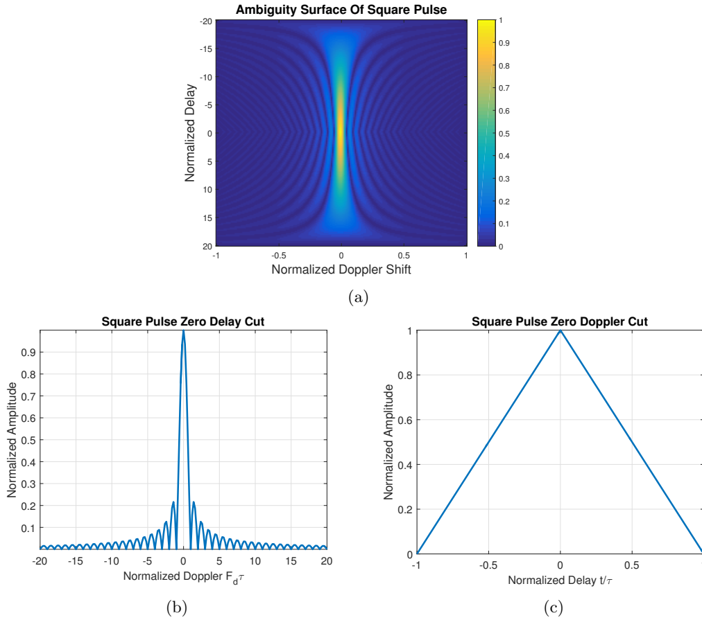
Figure 6: Rectangular pulse auto-ambiguity. (a) Ambiguity surface, (b) zero delay cut, (c) zero Doppler cut.
