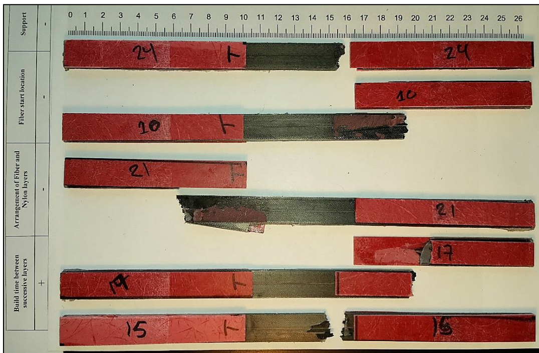
Figure 58. Test Point 2 After Testing
