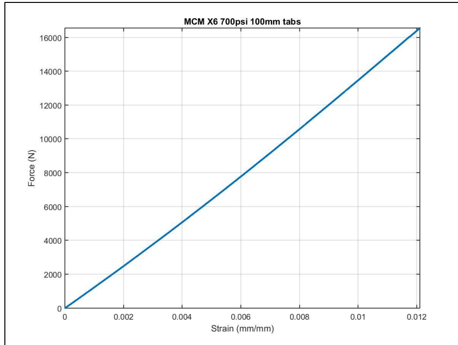
Figure 54. Force vs. Displacement for Calibration Sample Number 6 With 700psi Grip Pressure and 100mm × 15mm × 1.5mm Fiberglass Tabs
