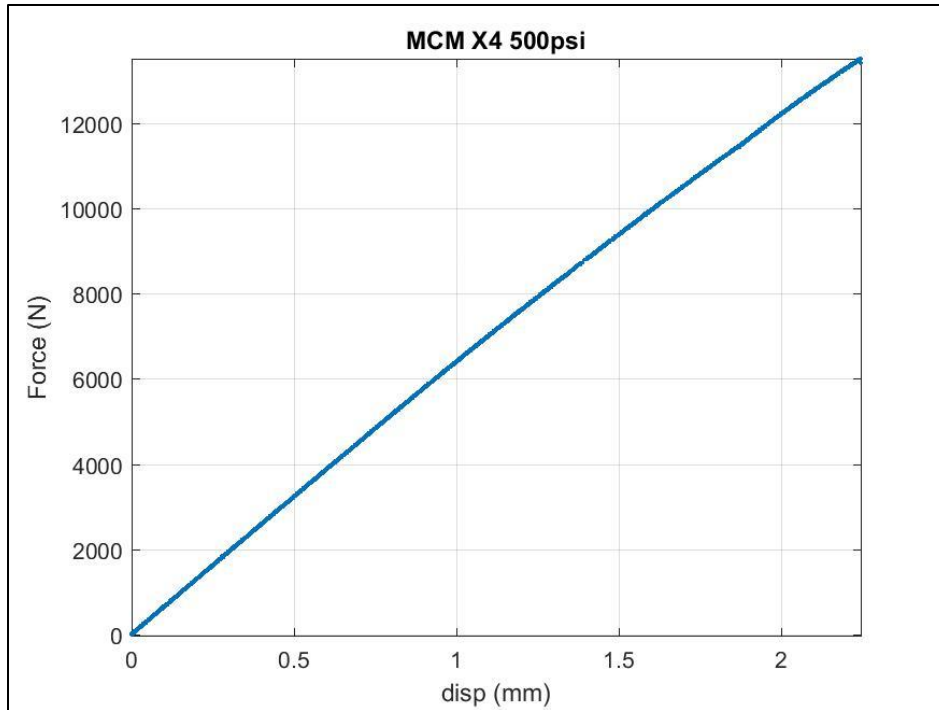
Figure 52. Force versus Displacement for Calibration Sample Number 4 With 500psi Grip Pressure and 50mm × 15mm × 1.5mm Fiberglass Tabs
