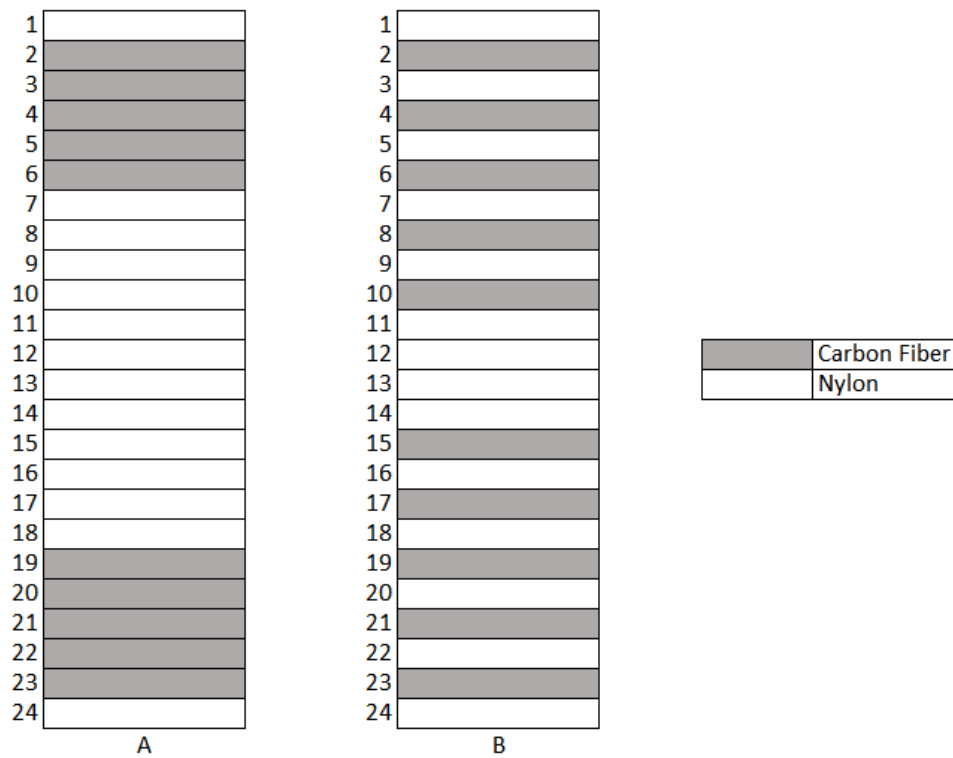
Figure 21. Two Fiber/Nylon Layup Sequence (A) Default, (B) Effect Setting
