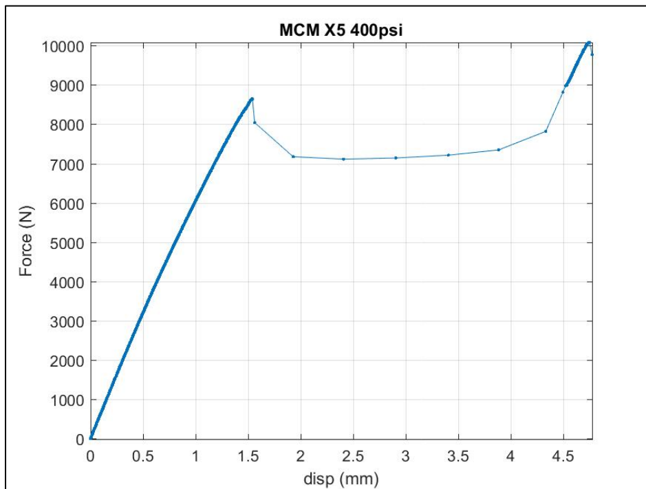
Figure 53. Force versus Displacement for Calibration Sample Number 5 With 400psi Grip Pressure and 50mm × 15mm × 1.5mm Fiberglass Tabs
