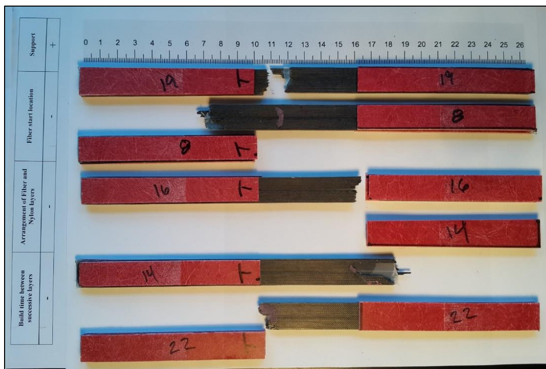
Figure 61. Test Point 5 After Testing
