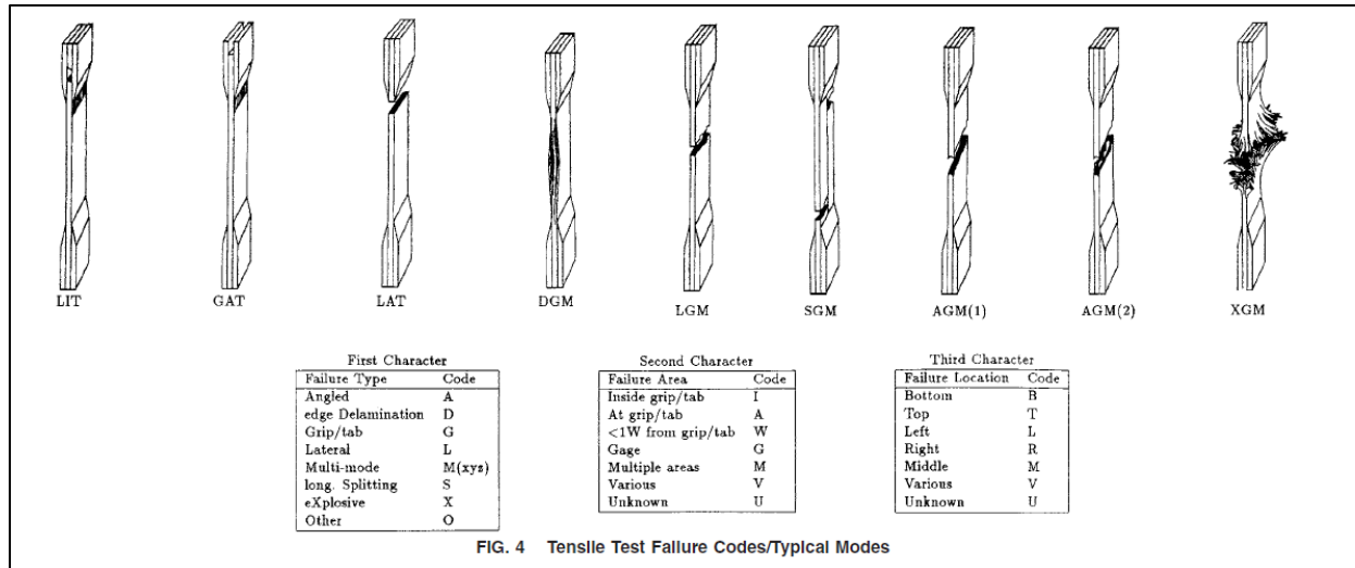
Figure 38. Tensile Tesnt Failure Codes/Typical Modes (ASTM Standard D3039/D3039M, 2014)
