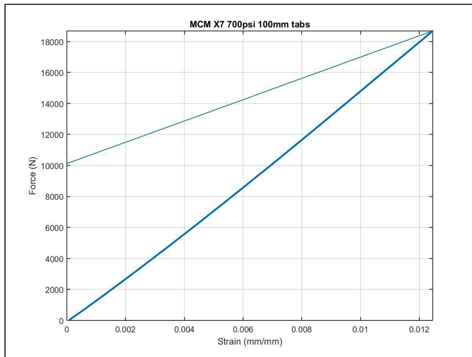
Figure 55. Force vs. Displacement for Calibration Sample Number 7 With 700psi Grip Pressure and 100mm × 15mm × 1.5mm Fiberglass Tabs
