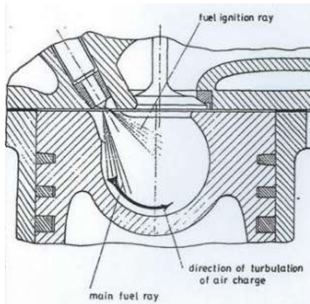
Figure 9 - Spherical Combustion Chamber in Multifuel Engine Piston (Elkothb, 1980)
