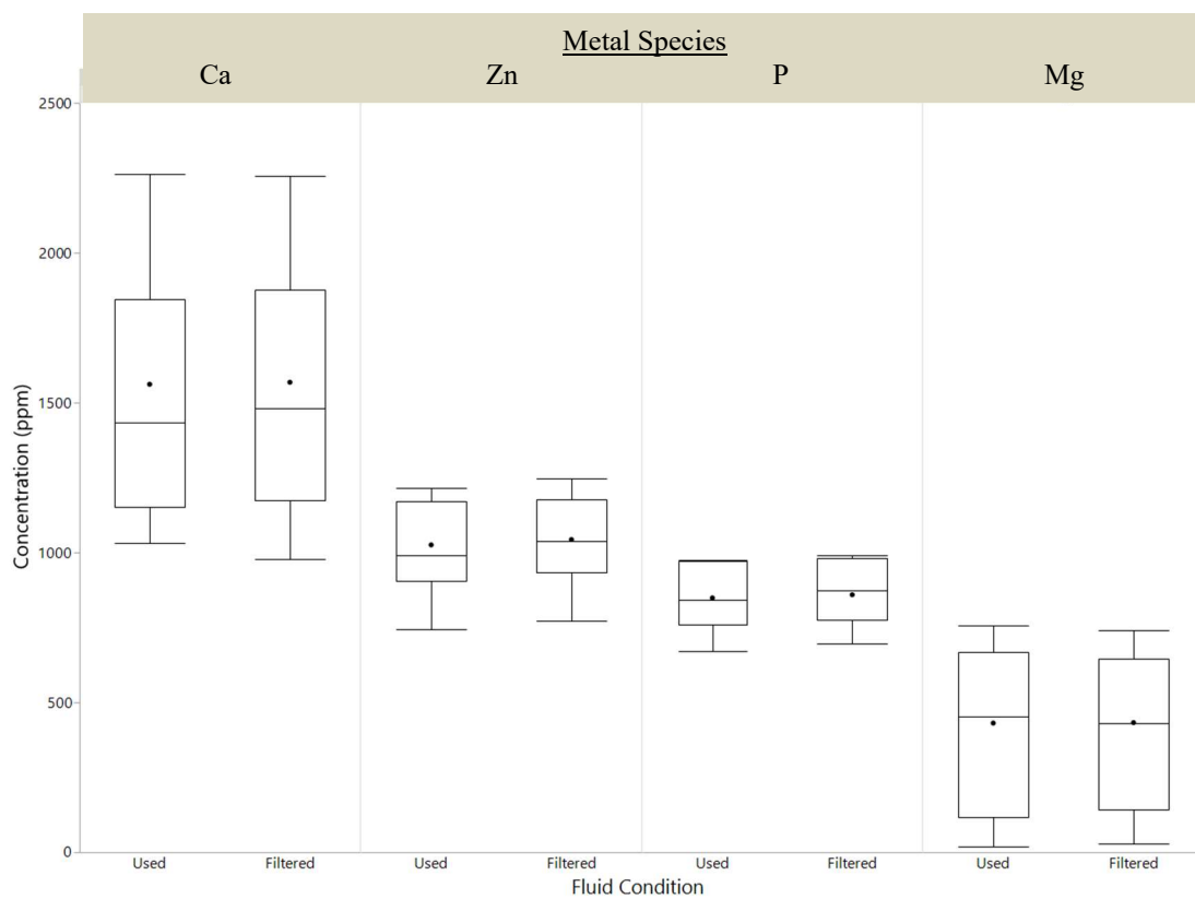
Figure 34 - Metals Filtering Comparison, Large Concentrations
