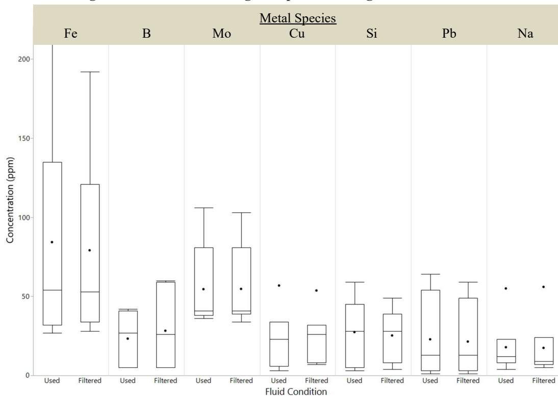
Figure 35 - Metals Filtering Comparison, Medium Concentrations
