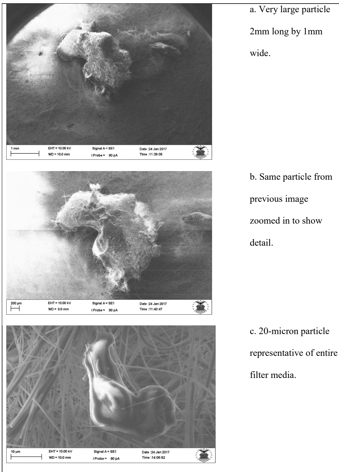
Figure 31 - Centrifuge Rotor Cap Residual Particulate Matter Viewed Under SEM
