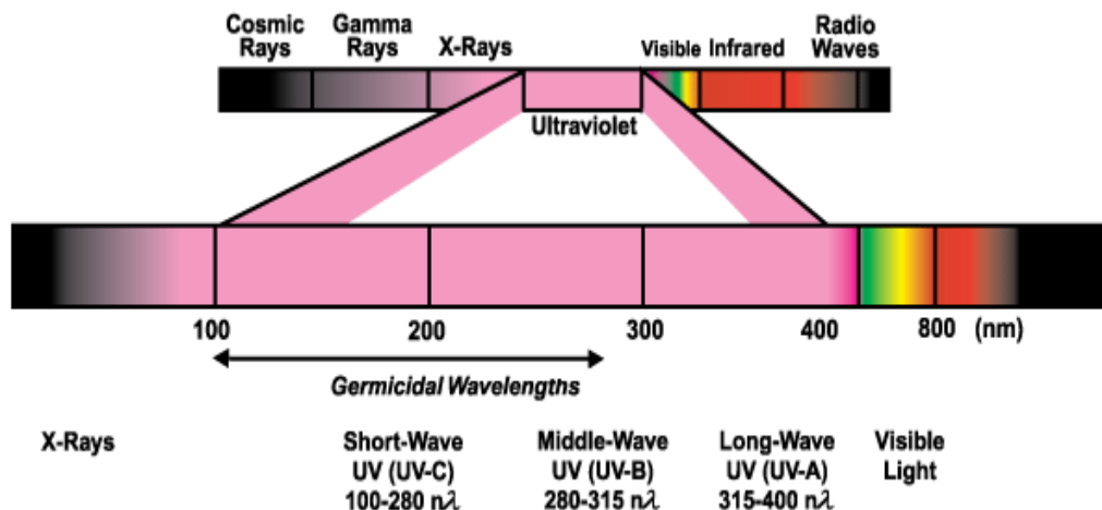
Figure 4: Electromagnetic Spectrum, UV-C Germicidal Wavelengths
