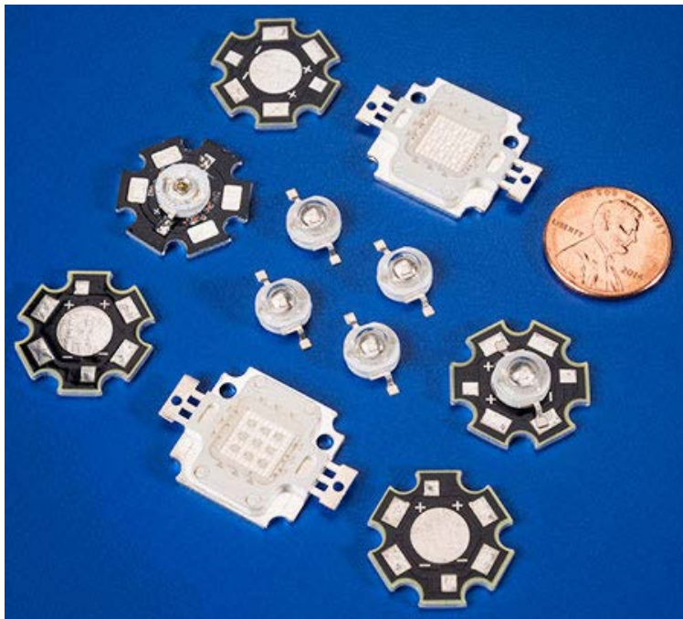
Figure 9: Ultraviolet Light Emitting Diode
