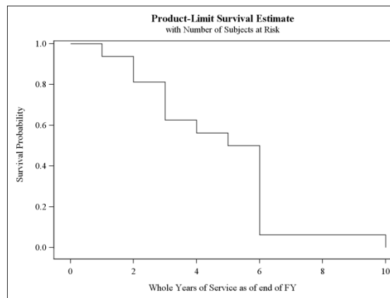
Figure 6. Example of 1A8X1M sustainment line using survival analysis
