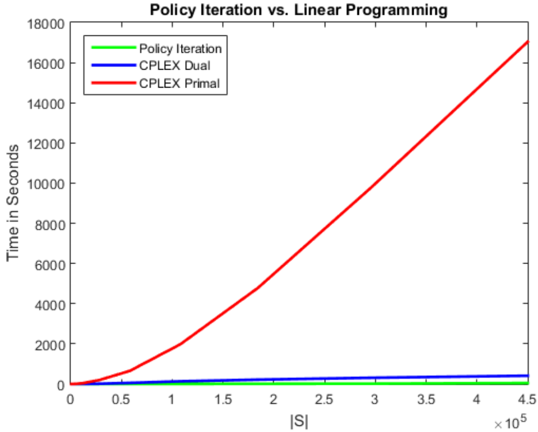
Figure 13. Policy Iteration vs Linear Programming
