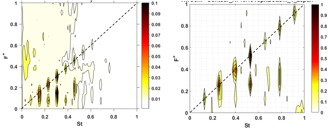
Figure 20: Contour plots of (a) PSD and (b) coherence spectra across the central \frac{1}{2} of the wake (1.5c) for select forcing frequencies at x/c=6 . The dashed line indicates a slope of one.
