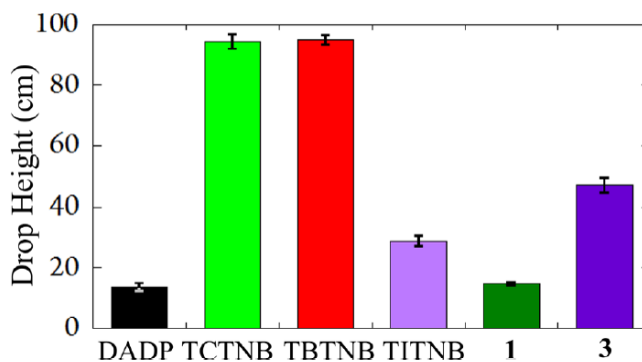
FIGURE 7 Relative impact sensitivity of explosive pure solids and cocrystals as h_{50\%} .
