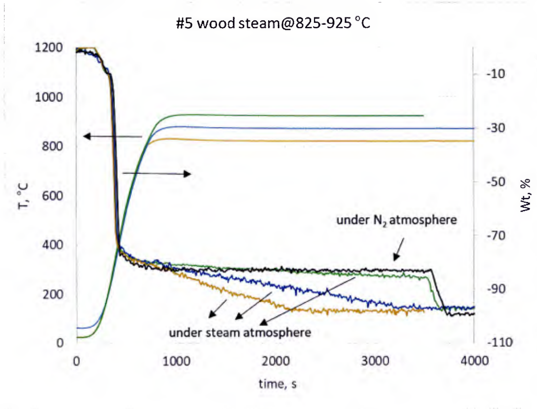
Figure 3.2a.3 Typical TGA graph showing reactivity in steam for a wood sample heated at 100 °C min -1 to a final temperature of 825, 875, and 925°C as indicated in the graph (yellow, blue and green curves respectively). Black curve is wood sample under N 2 (no steam), heated at 100 °C min -1 to a final temperature 925°C.
