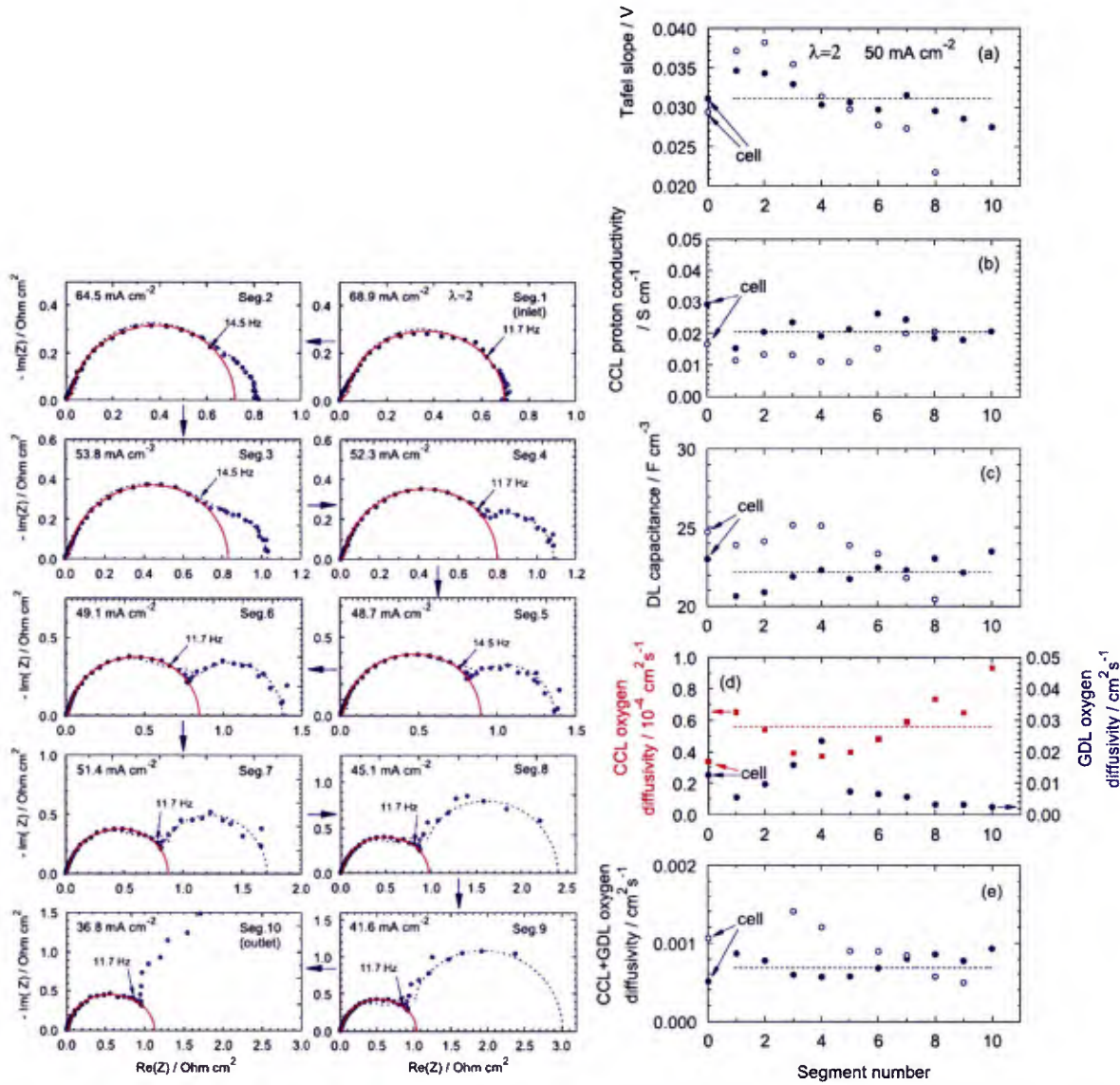
Figure 2.1.23. Experimental impedance spectra (symbols) and fitted mathematical models (lines) for an air stoichiometry of 2 and 0.05 \text{ A cm}^{-2} (left). The solid lines correspond to the 1D model whereas dash lines relate to the quasi-2D model. Fitted parameters for segments 1-10 (right). Filled circles data points were obtained with the 1D model whereas open circles data points were derived with the quasi-2D model. Dash lines refer to average 1D model parameters. Parameters obtained by fitting impedance spectra for the entire cell are indicated by data points for the zero segment number.
