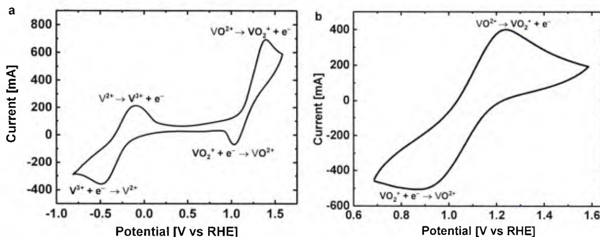
Figure 2.1.15. CVs recorded at 20 mV s -1 and 25 °C for the V(IV) electrolytes after charging with graphite rod electrodes. Negative (a) and positive (b) electrolytes.
