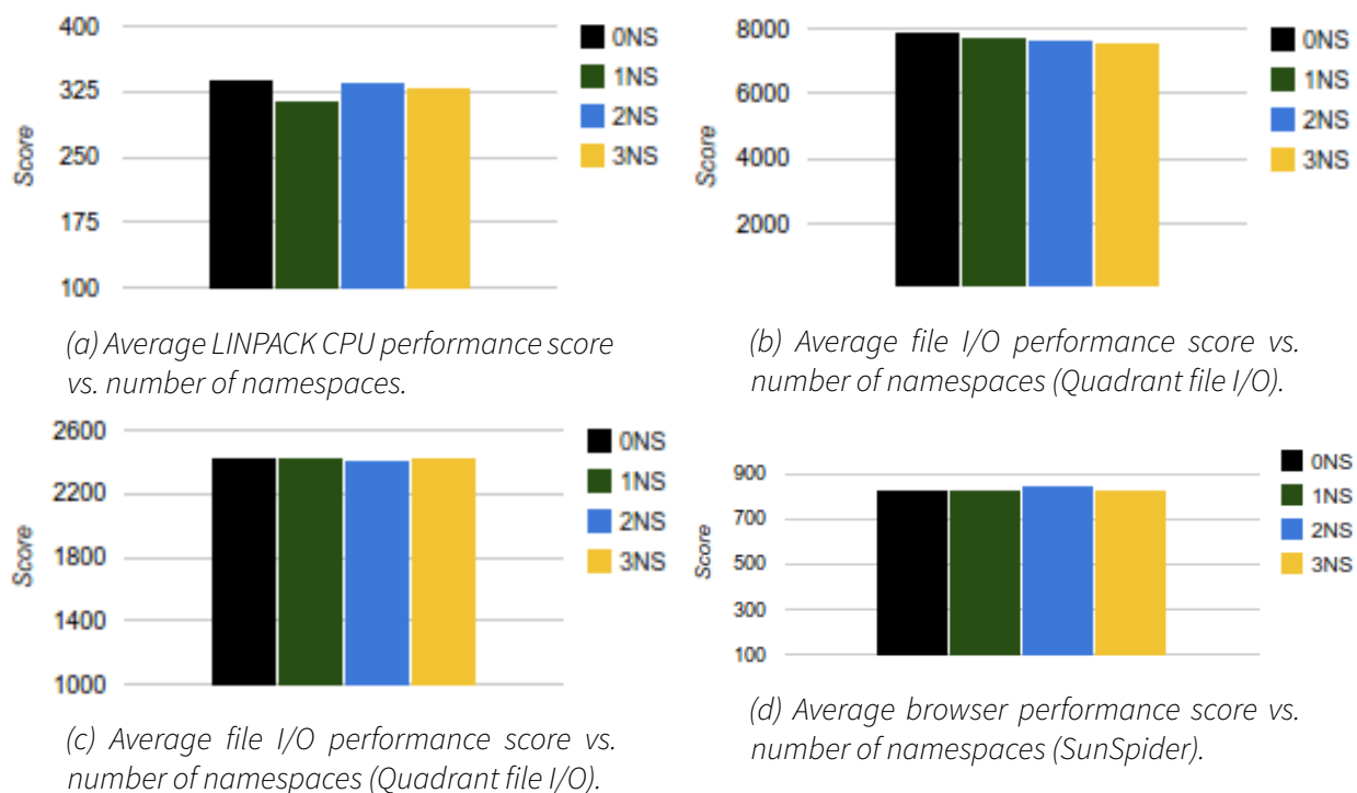
Figure 5.13: Benchmarking results for 0-, 1-, 2- and 3-namespace configurations.
