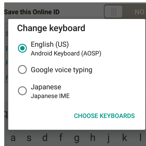
(b) Critical banking app running in alternate IME namespace, showing only built-in input methods as selection options.
