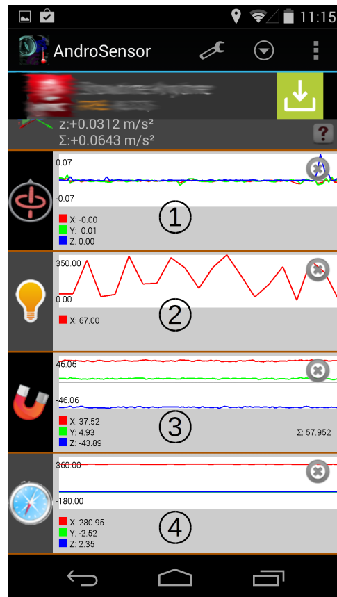
(b) AndroSensor running in 2 nd alternative sensor namespace showing normal traces for gyro (①), magnetic (③), and orientation (④) sensors, and random trace for light sensor (②).
