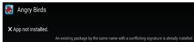
Figure 3.5: New package installation is denied due to existing package with the same name but different signature.
