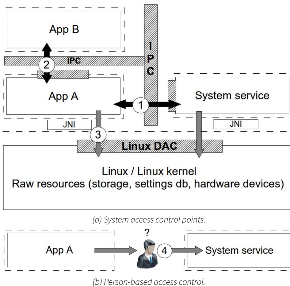
Figure 3.3: Android communication paths showing access control points.
