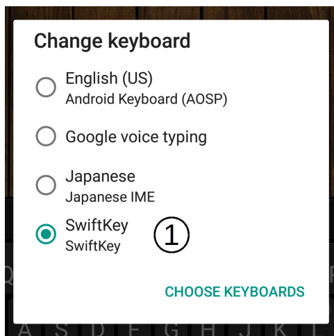
(a) Non-critical app running in global IME namespace, showing all input methods, including a 3 rd party (1), as selection options.
