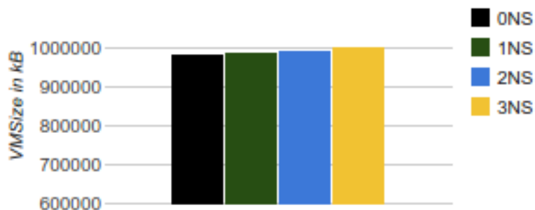
Figure 5.14: Average memory footprint in kB (VmSize) for 0-, 1-, 2- and 3-namespace configurations.
