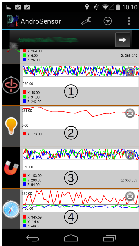
(a) AndroSensor running in 1 st alternative sensor namespace showing normal trace for light sensor (②), and random traces for gyro (①), magnetic (③) and orientation (④) sensors.
