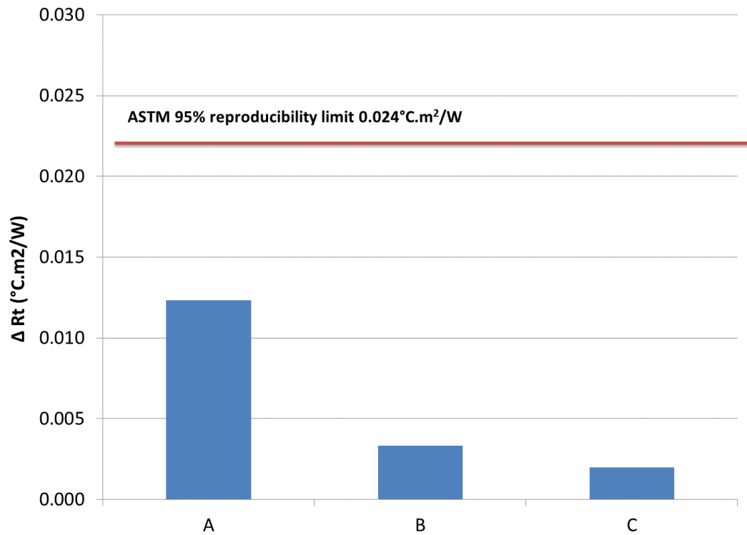
Figure 8. Differences in thermal insulation according to ASTM 95% reproducibility standard
