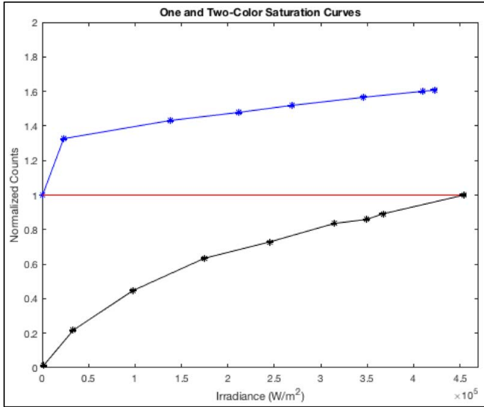
Figure 31. One- and two-color saturation curves for uranium using a known sample; CRM125A. Black: 396 nm alone. Blue: 406 nm varied with 396 nm held constant and normalized to 1 from the 396 nm laser. Red: normalization count line for 406 nm saturation curve.
