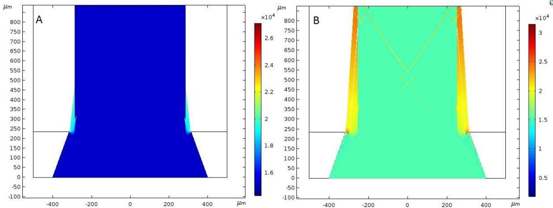
Figure 20. Ionization comparison (a) blank and (b) CNT growth models at 250 V
