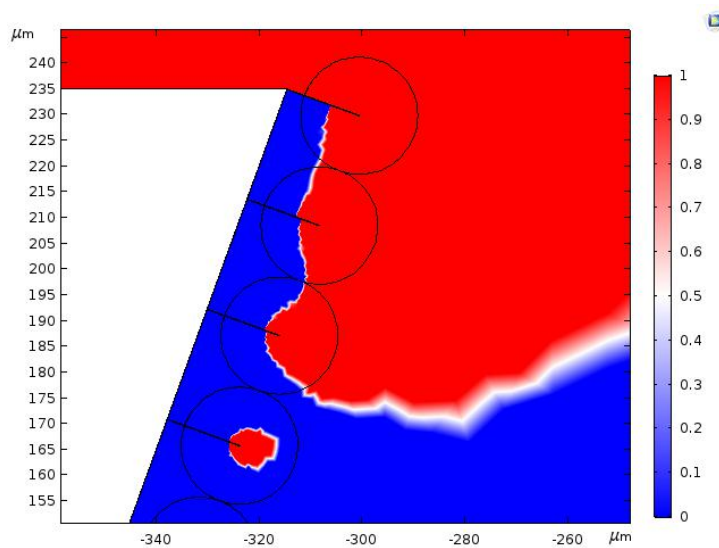
Figure 19. Zoomed electric field of CNT growth sample at 350V
