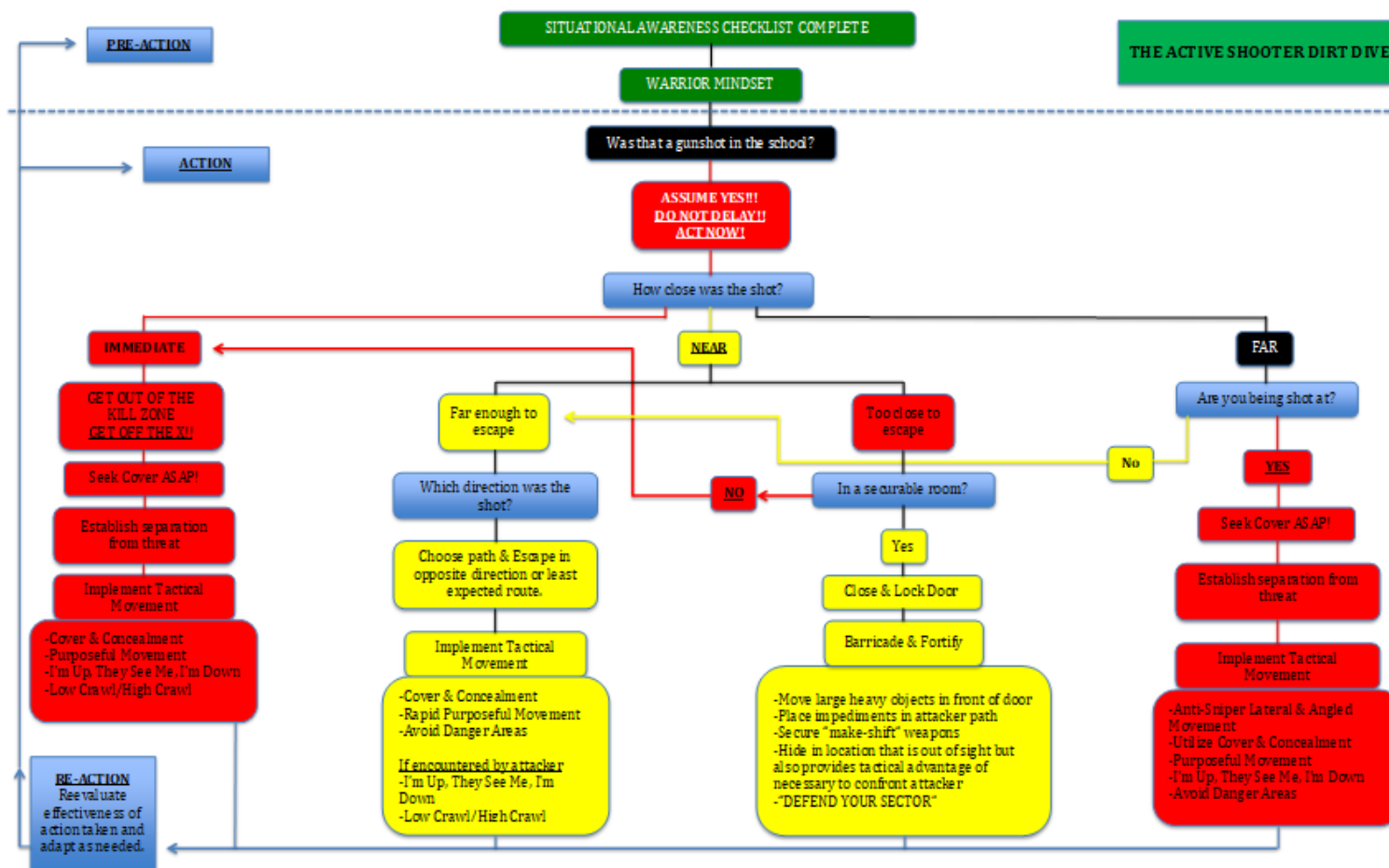
Figure 15. The Active Shooter Dirt Dive 407
