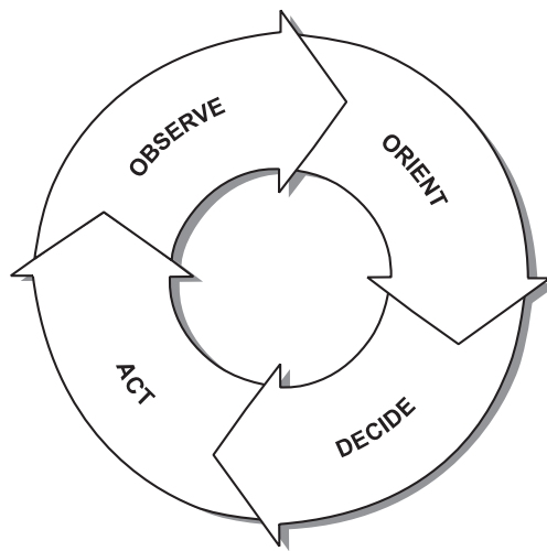
Figure 8. The Observe, Orient, Decide, and Act Loop 306
