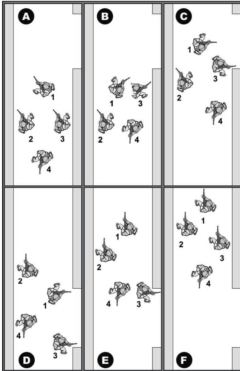
Figure 12. Clearing Hallway Junctions at “a ‘T’ Intersection when Approaching along the ‘Cross’ of the ‘T’” 378
