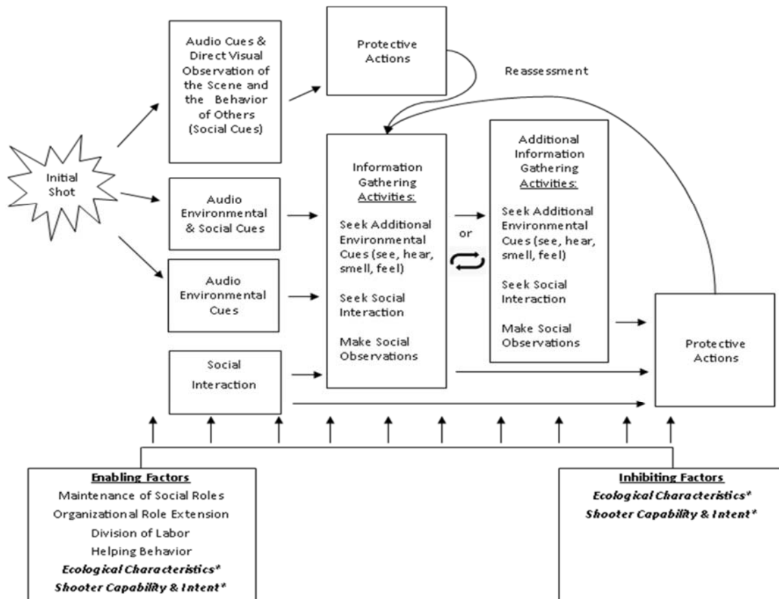
Figure 6. The Socio-Behavioral Response of Survivors to Campus Active Shooter Events 289
