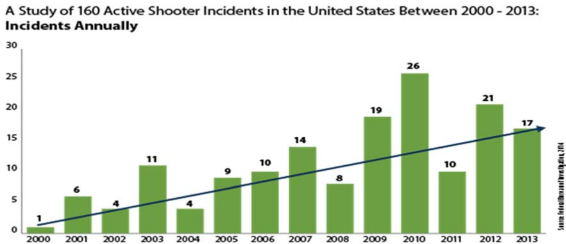
Figure 3. Active Shooter Incidents: Incidents Annually 87
