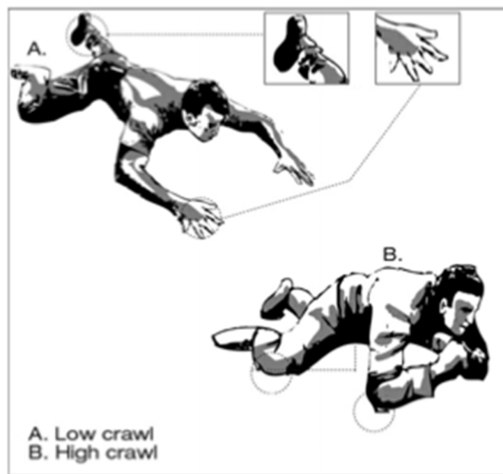
Figure 11. High Crawl versus Low Crawl 374
