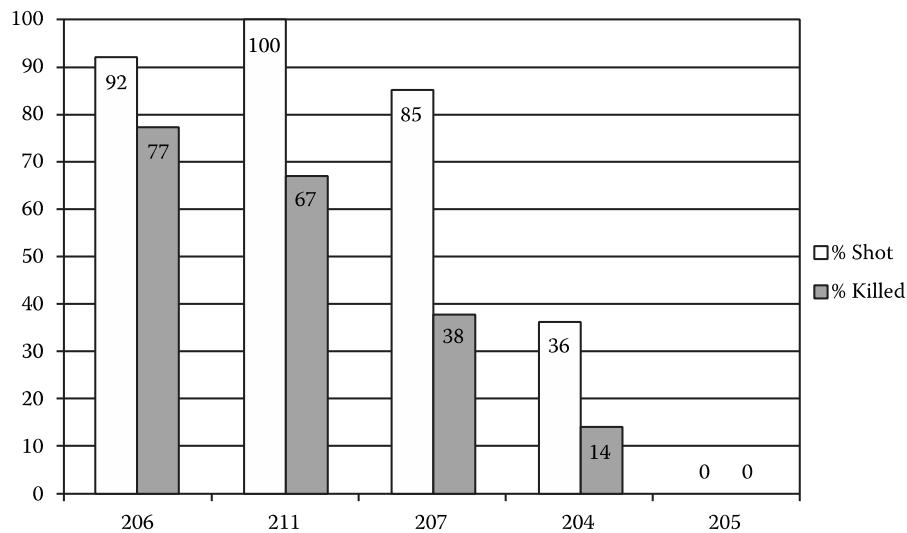
Figure 4. Number of People Shot and Killed at Virginia Tech 100
