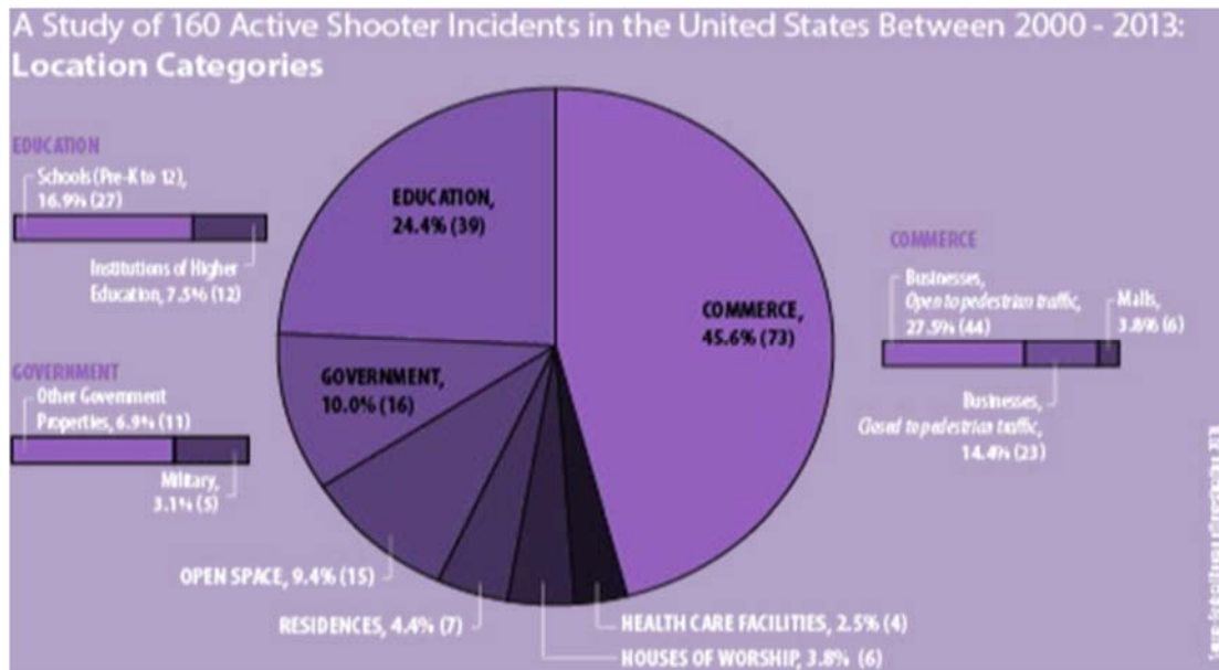
Figure 2. Active Shooter Incidents: Location Categories 86
