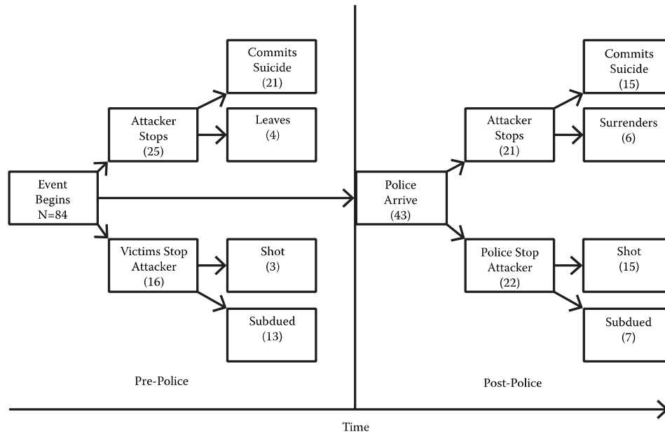
Figure 5. Resolution of Active Shooter Events in the United States (2000–2010) 192
