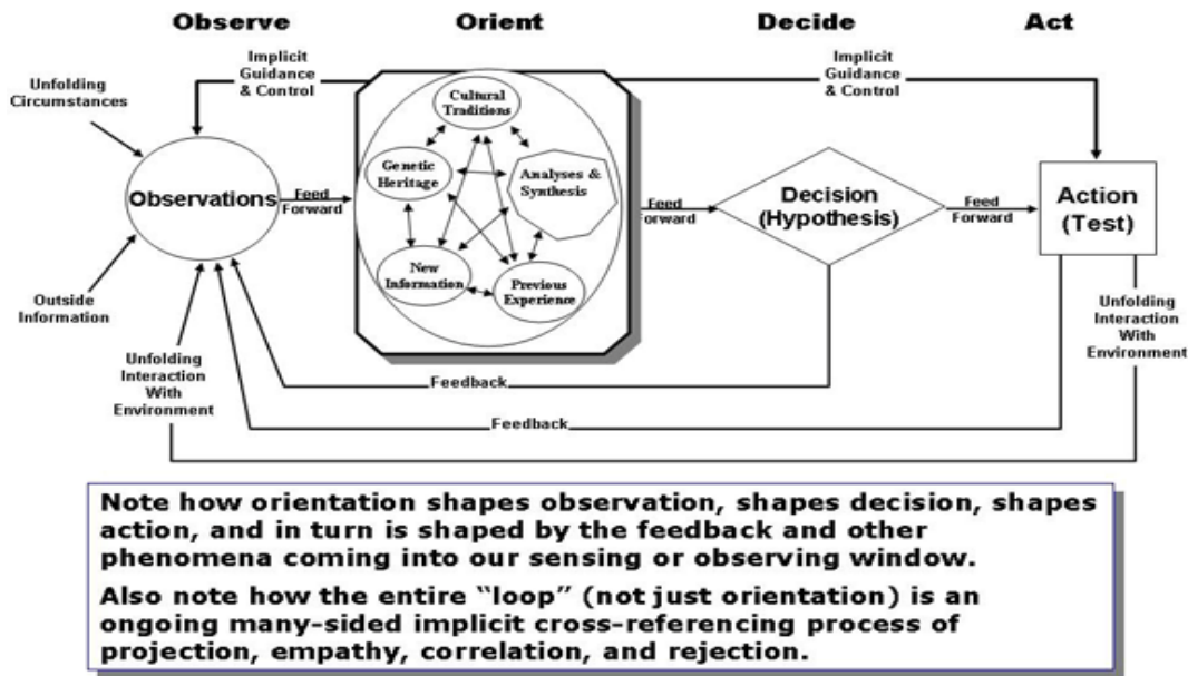
Figure 7. Boyd's OODA Loop 305
