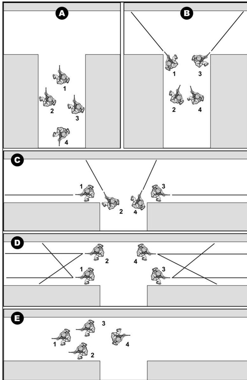
Figure 13. Clearing Hallway Junctions at “a ‘T’ Intersection when Approaching from the Base of the ‘T’” 379
