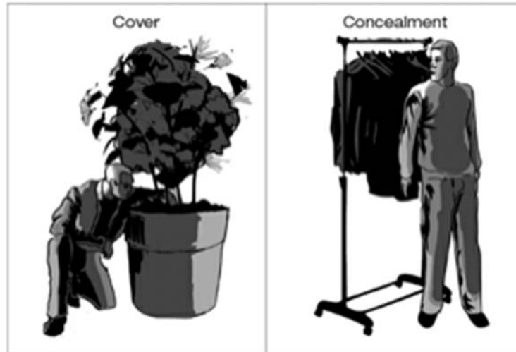
Figure 9. Cover versus Concealment 341
