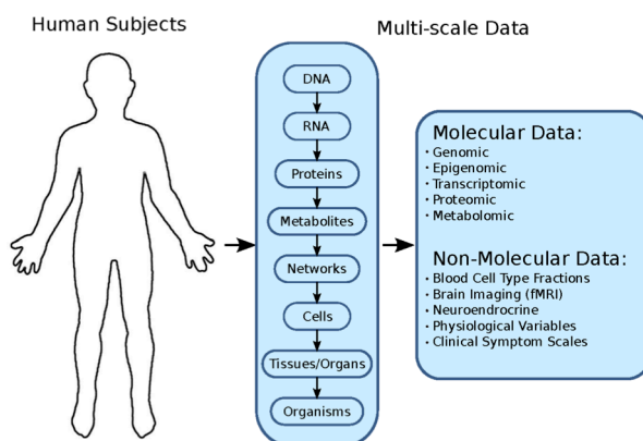
Figure 1.1 Systems biology approach for the study of PTSD: a multitude of data types can be experimentally collected by probing biological systems at different scales. This wealth of data is then further processed by employing mathematical and computational techniques ( e.g. , statistics, machine learning, computational modeling) to gain insight into the system under study (from [3]).
