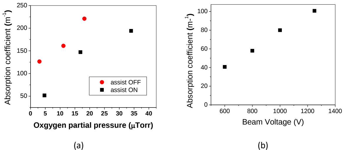
Figure 1: Absorption coefficient (at \lambda=1.064 \mu\text{m} ) vs. (a) oxygen partial pressure and (b) beam voltage. The assist beam in (a) refers to a second ion beam that improves mobility on the growth film surface.
