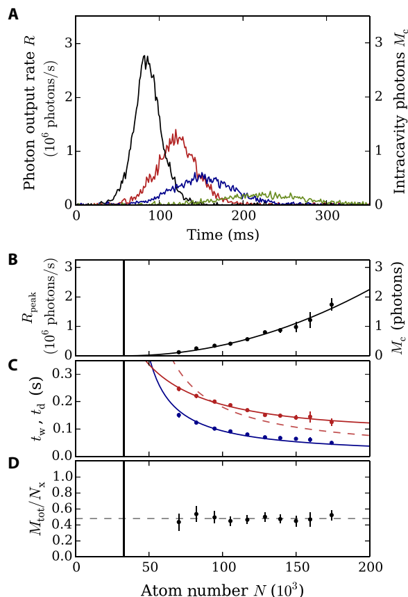
Fig. 2. Spontaneously generated superradiant pulses. (A) Representative single time traces of photon output rate R for pulses at different atom numbers N \approx 100 \times 10^3 (green), 125 \times 10^3 (blue), 150 \times 10^3 (red), and 200 \times 10^3 (black). The equivalent average intracavity photon number is calculated on the right as M_c = R/\kappa . (B) Peak photon output rate, R_{\text{peak}} , versus initial total atom number. The black line is a quadratic fit to the output power. We observe a horizontal offset in the fit, indicating a threshold atom number N_t [black vertical line in (B) to (D)]. The threshold results from decoherence and atom loss and is a signature of lasing that would not be present for single-atom emission. (C) FWHM pulse duration t_w (blue) and delay of peak power t_d (red) versus initial total atom number. The blue line is a fit to the predicted functional form for the pulse duration, with N_t determined from the fit to R_{\text{peak}} . The dashed red line is a fit to the pulse delay, assuming that threshold is due to atomic homogeneous broadening without atom loss. The solid red line is a fit to the pulse delay, assuming that the threshold is set only by atom loss from the lattice. (D) The ratio of emitted photons M_{\text{tot}} to the number of atoms in excess of threshold N_x plotted versus atom number. The dashed line is the average ratio, showing that 48% of the atoms in excess of threshold participate in the superradiant pulse, largely independent of N .
