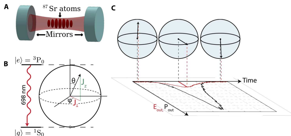
Fig. 1. Experimental overview. (A) Our system consists of an ensemble of up to N = 2.5 \times 10^5 laser-cooled ^{87}\text{Sr} atoms confined in a magic-wavelength optical lattice within a high-finesse ( F = 2.4 \times 10^4 ; linewidth, \kappa = 2\pi \times 160 kHz) optical cavity. (B) The atoms undergo pulsed superradiant lasing on the ^3\text{P}_0 -to- ^1\text{S}_0 optical clock transition that has a natural decay time of 150 s or an equivalent linewidth of 1 mHz. The state of the atomic ensemble can be represented by a collective Bloch vector (explained in the text). (C) Representation of a superradiant pulse on the Bloch sphere. The Bloch vector behaves like a highly damped pendulum that starts inverted at the north pole of the Bloch sphere (excited state). Quantum fluctuations disturb the system from its unstable equilibrium position, causing the Bloch vector to swing down the Bloch sphere, emitting peak radiation at the equator, and ultimately relaxing to the south pole (ground state), as inversion is lost. The radiated electric field (red trace) is proportional to the perpendicular projection of the Bloch vector, J_{\perp} , which at its peak is proportional to N . The radiated power (black trace) is proportional to the square of the radiated electric field, and at its peak is therefore proportional to N^2 . This is one way to understand the origin of the collective enhancement in emission rate. The black output power trace on the projection plane is actual data.
