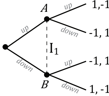
Figure 1. Example extensive form game with imperfect information. Play begins at the leftmost decision node. The first player selects a direction—either up or down. The second player cannot distinguish between state A and state B because they are both members of the information set I_1 .
