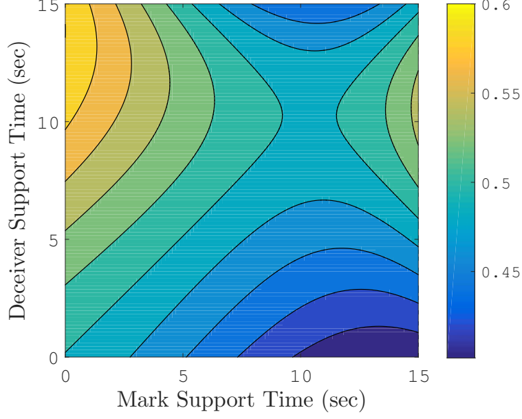
Figure 8. Deceiver Payouts for Missile Support Time game. The payouts for the mark and deceiver are nearly symmetric. The game exhibits a pure strategy Nash equilibrium wherein both players support for ten seconds.
