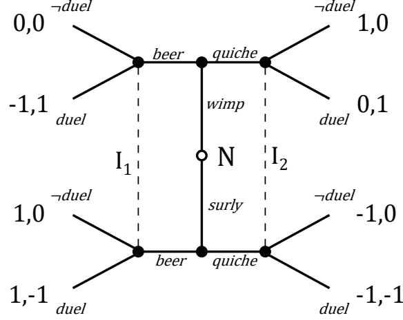
Figure 2. Wimp or Surly: the first Signaling game. Play begins when Nature (N) selects a type t for A, either wimp or surly. At the next decision node, A selects either beer or quiche as the signal (S). B observes the signal, but the information sets I_1 and I_2 make it impossible to discern t . So, B selects an action knowing only what A ate for breakfast.
