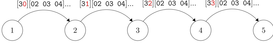
Figure 26. Z-Wave mesh topology routing. Node 0x01 sends a routed packet to Node 0x05. The hop counter is steadily incremented until the final destination is reached.
