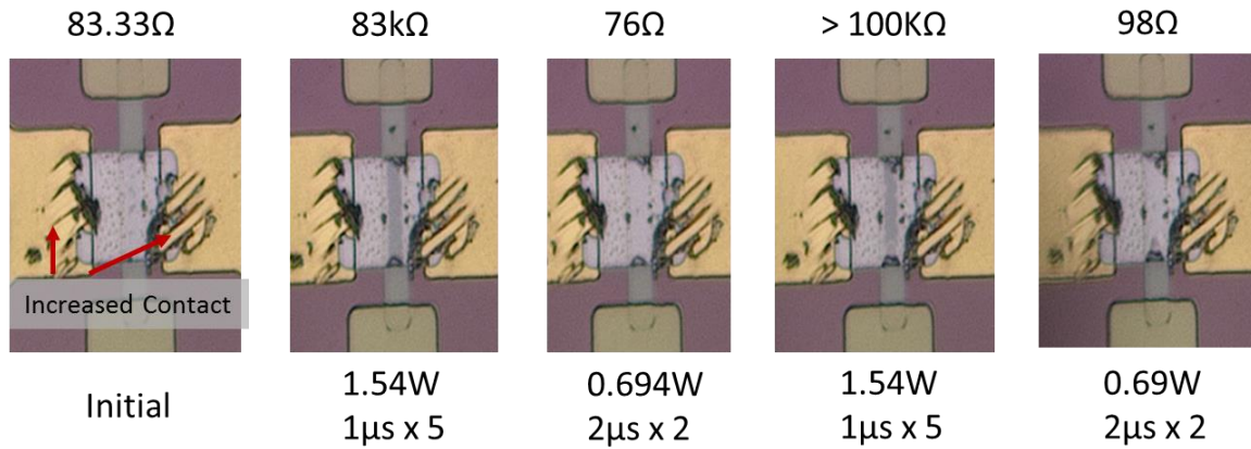
Fig. 72. Variation of germanium telluride resistance with successive voltage pulses. The resistances shown at the top of each image were formed after the pulses at the bottom of each image were transmitted. The physically enhanced contact surfaces are marked with red arrows in the initial image. In the “>100kΩ” measurement, the resistance slightly exceeded the maximum measurable resistance of the low-voltage resistance measurement setup.
