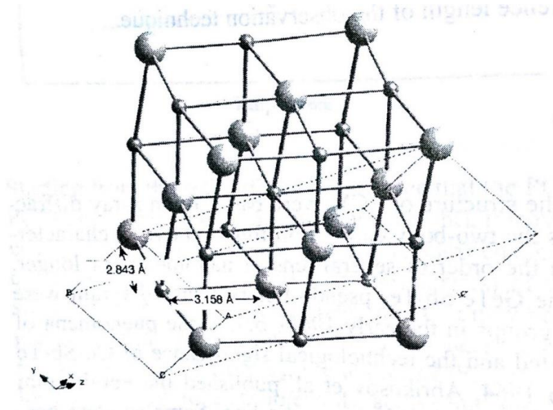
Fig. 29. GeTe has a distorted NaCl crystal structure [99].
