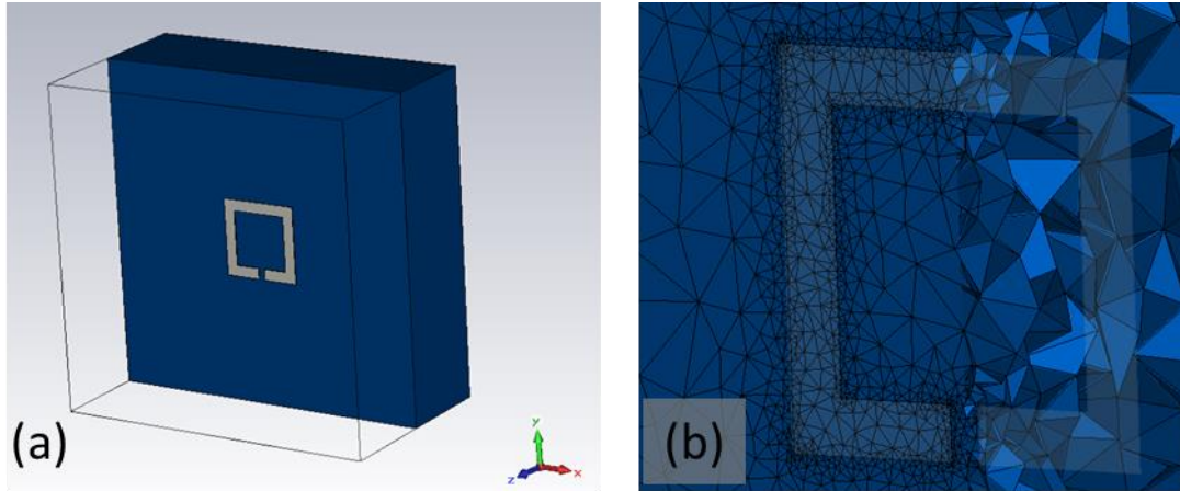
Fig. 36. SRR model. An overview of the model is shown in (a). A slice showing the tetrahedral meshing of the model is shown in (b).
