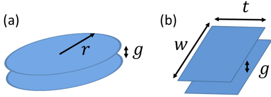
Fig. 16. Dimensions used for capacitance calculations of (a) two circular and (b) two rectangular plates
