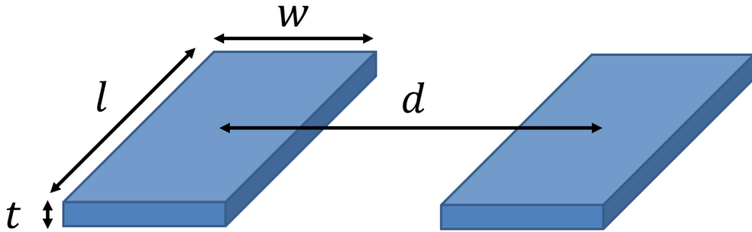
Fig. 14. Labeled dimensions of an inductive bar pair.
