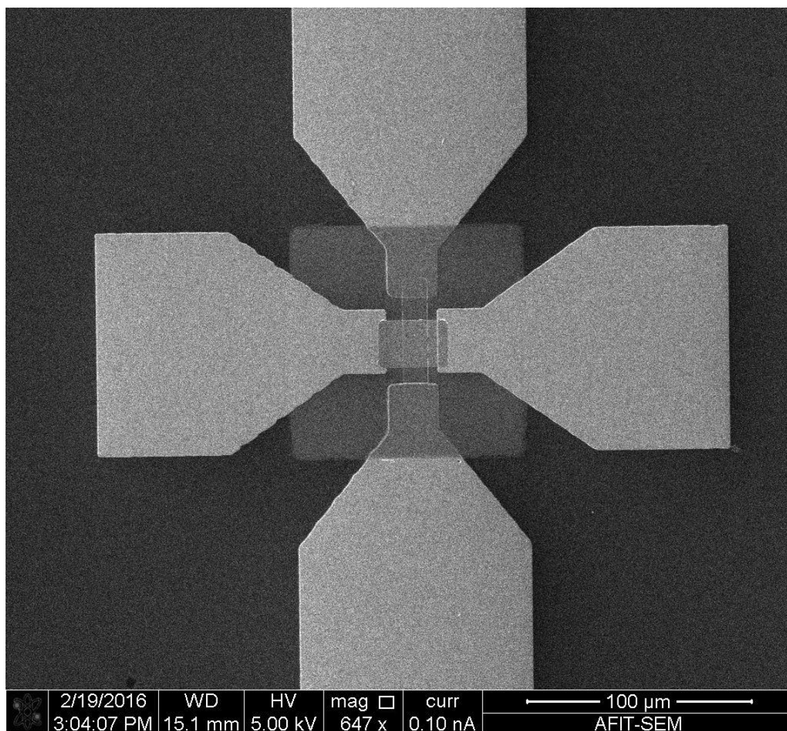
Fig. 70. A scanning electron microscope image of a finished indirect heating device
