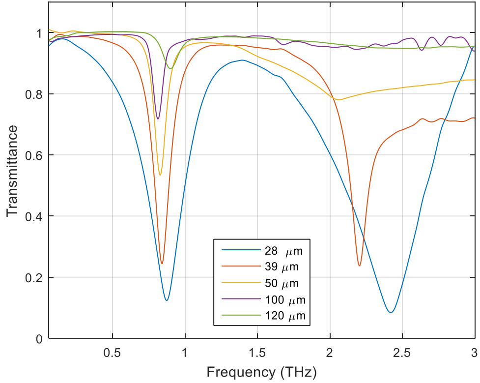
Fig. 54. Variations of transmission on periodicity of split-ring resonators on 1mm intrinsic silicon.
