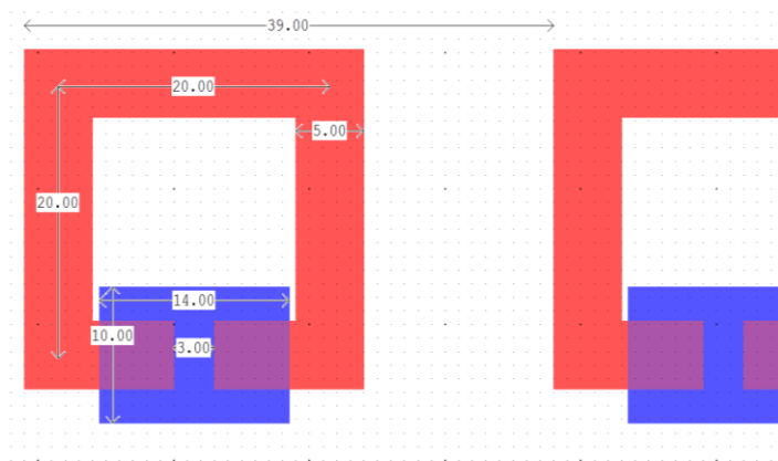
Fig. 95. Split-ring resonator elements with germanium telluride rectangles (blue) in their capacitive gaps, shown with dimensions.
