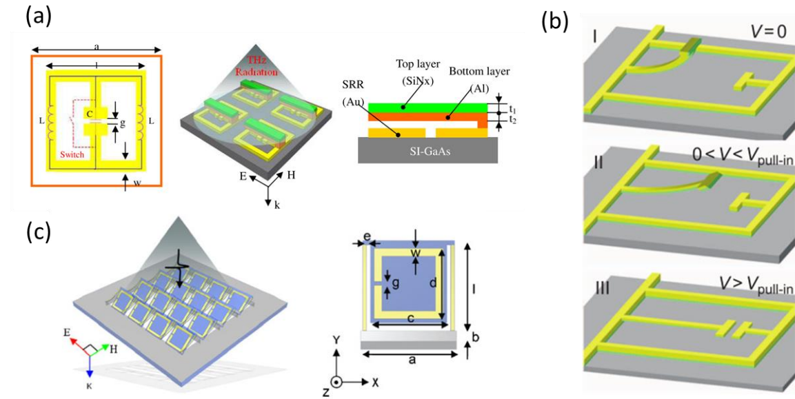
Fig. 23. Various microelectromechanical systems (MEMS) incorporated, tunable split-ring resonator (SRR) elements operating in the terahertz (THz) frequency range. In (a), modulation of a THz SRR is shown using bi-material cantilevers [42]. The design in (b) uses bi-material cantilevers for the inner capacitive gap arms of THz SRRs, achieving modulation when these arms are deflected [84]. The third design in (c) shows structurally tunable THz SRRs using bi-material cantilevers to bend the entire array in different directions [158]
