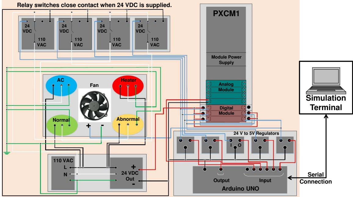
Figure 3. Apogee HVAC system schematics.
