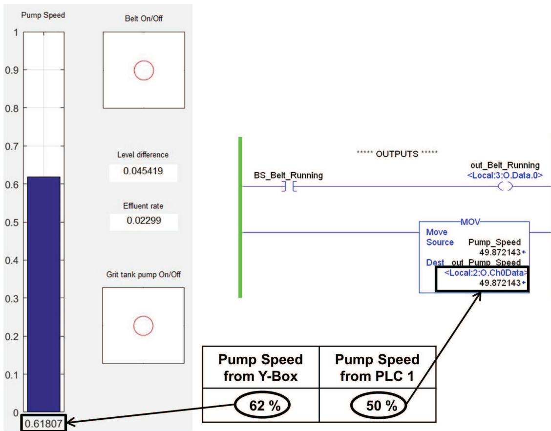
Figure 17. Attack 1 example.
