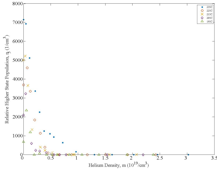
Figure 7. The densities of the highest excited states vs Helium density at different temperatures. The \bullet represents taken collect at a cell temp of 235^{\circ}\text{C} . The \circ is at 225^{\circ}\text{C} , \times is 215^{\circ}\text{C} , \diamond is for 205^{\circ}\text{C} , and the \triangle is for 195^{\circ}\text{C} . As the total Rubidium density increases, the Helium pressure necessary to quench all of the tranistions from the highest energy levels increases as well.
