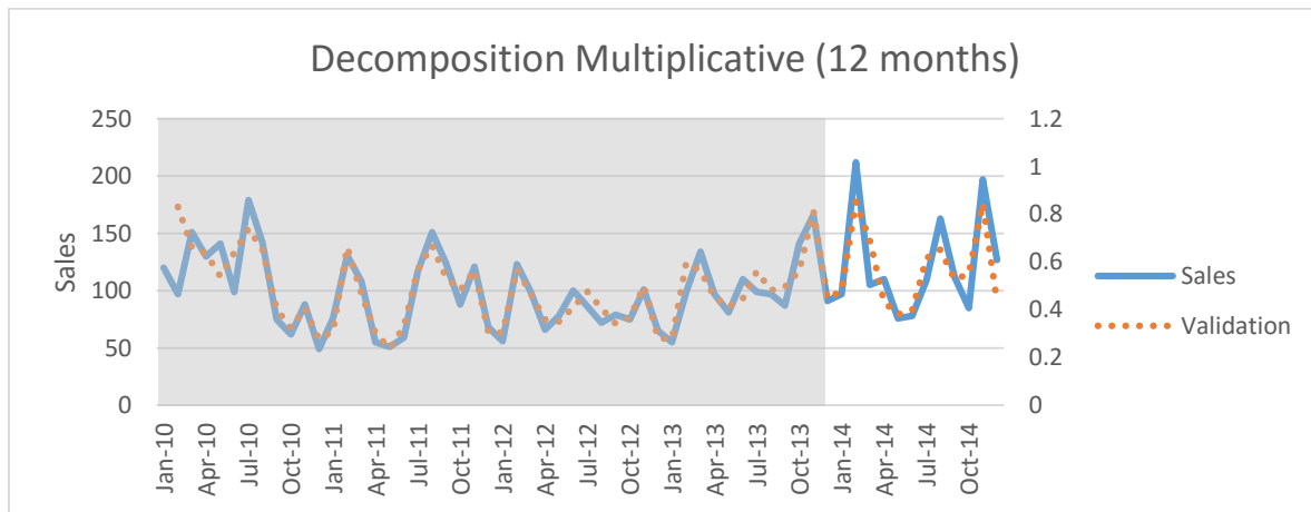
Figure 10. Graphical output of forecasted values
