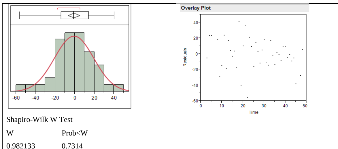
Figure 3. Validity assumptions for coat forecasting residuals
