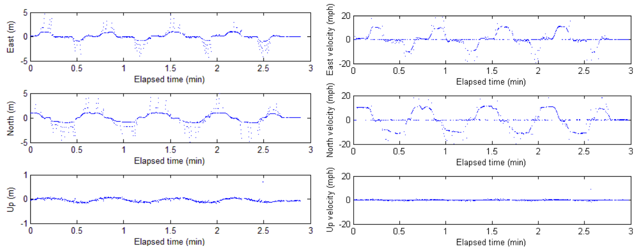
Figure 4-20: Test #5 position solution error and velocity
