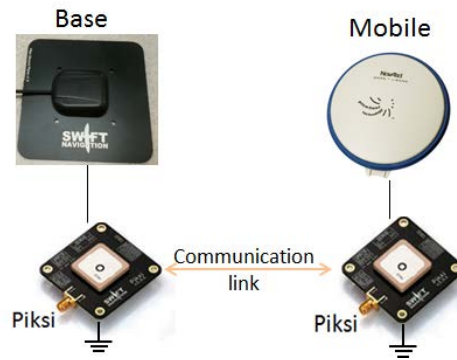
Figure 4-26: Test #3 setup [20] [22]
