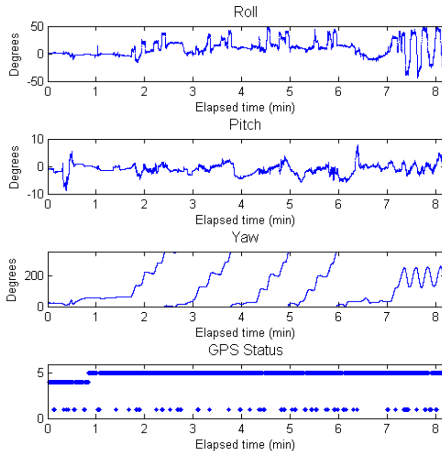
Figure 4-39: Piksi GPS status
