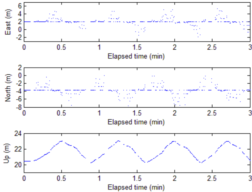
Figure 4-30: Test #7 position solution error after 0.2s offset applied
