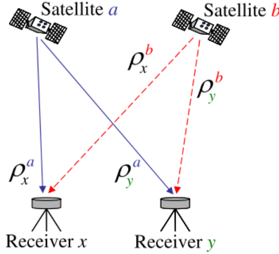
Figure 2-2: Double Difference Schematic [25]
