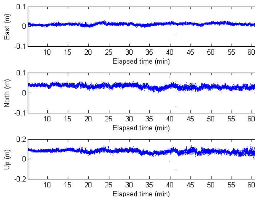
Figure 4-18: Test #1 position solution error during RTK lock
