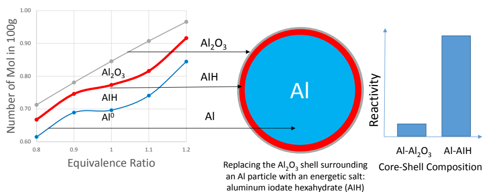
Figure 17. AlH replacement of Al 2 O 3 passivation layer. All lines represent the moles of Al in 100 grams of mixture via XRD analysis.
