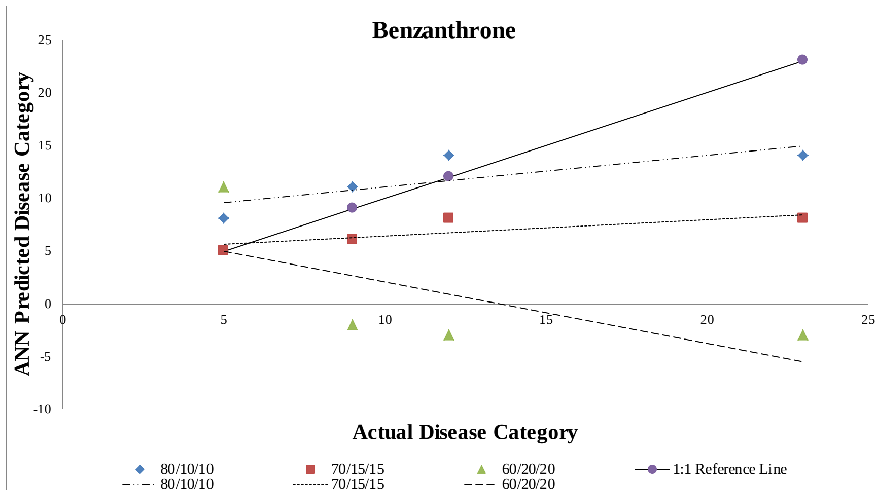
Figure 13: Benzanthrone
