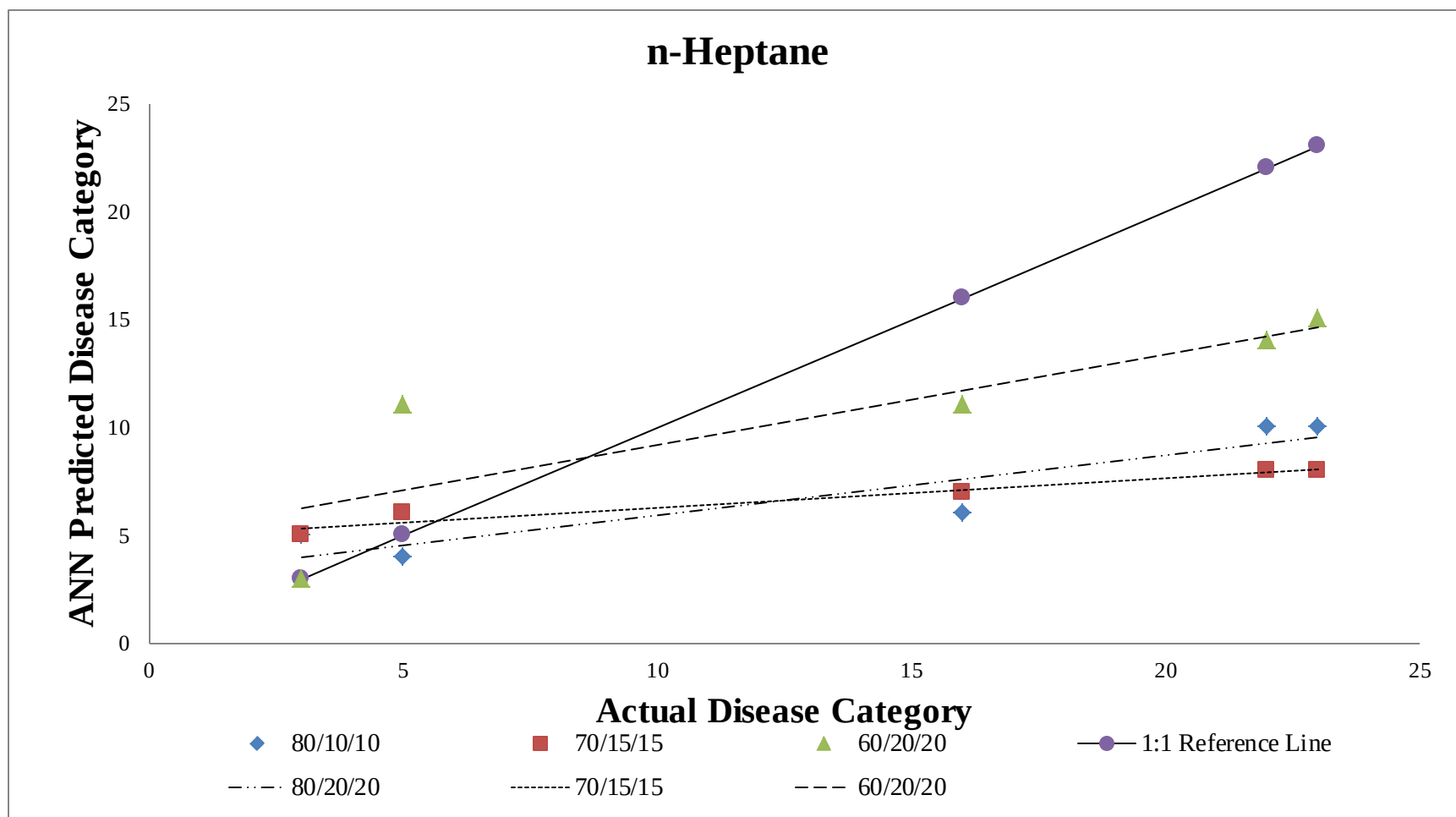
Figure 15: n-Heptane
