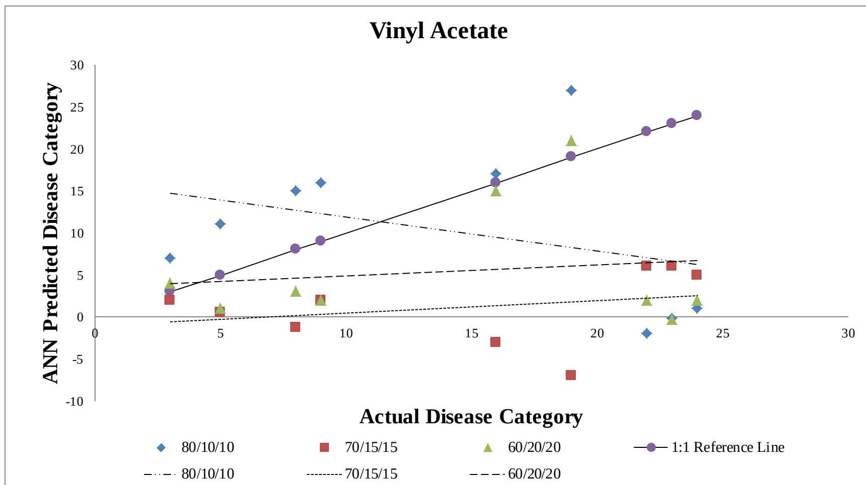
Figure 21: Vinyl Acetate
