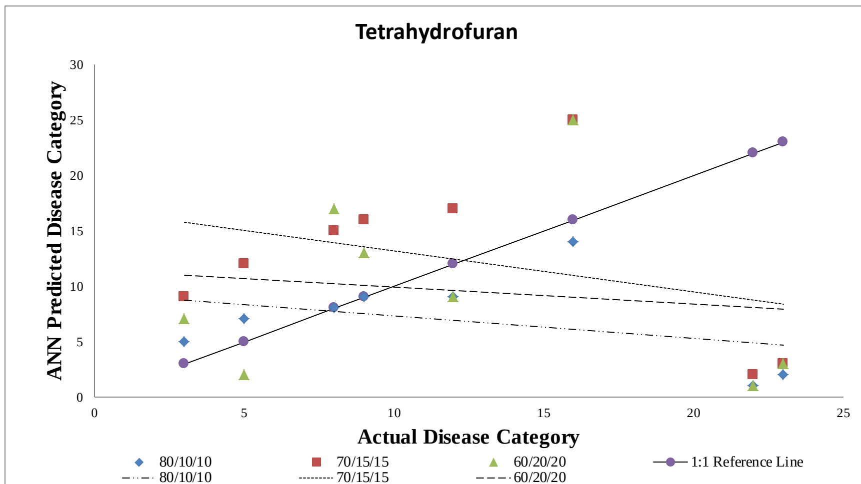
Figure 19: Tetrahydrofuran
