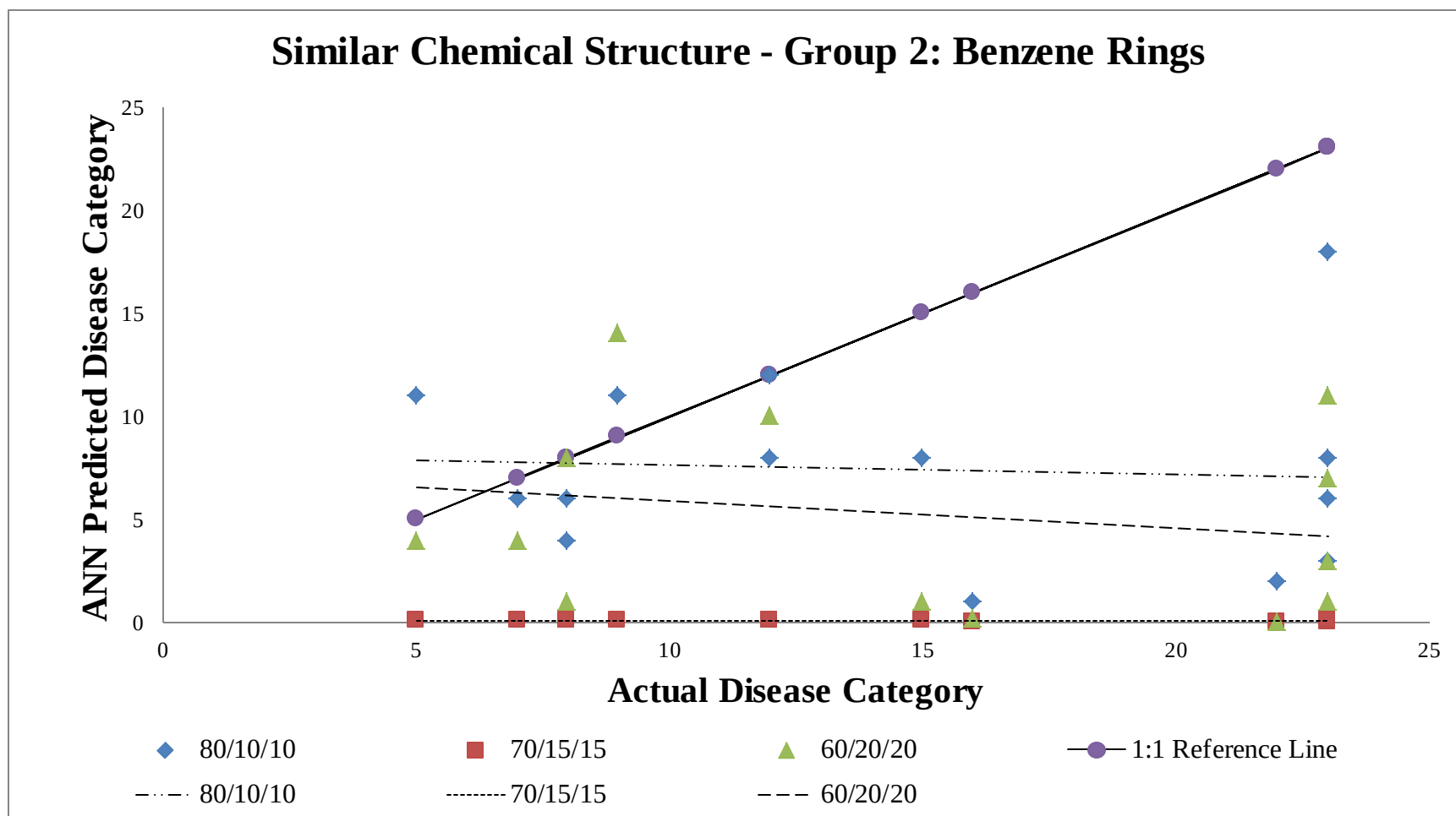
Figure 6: Similar Chemical Structure - Group 2: Benzene Rings
