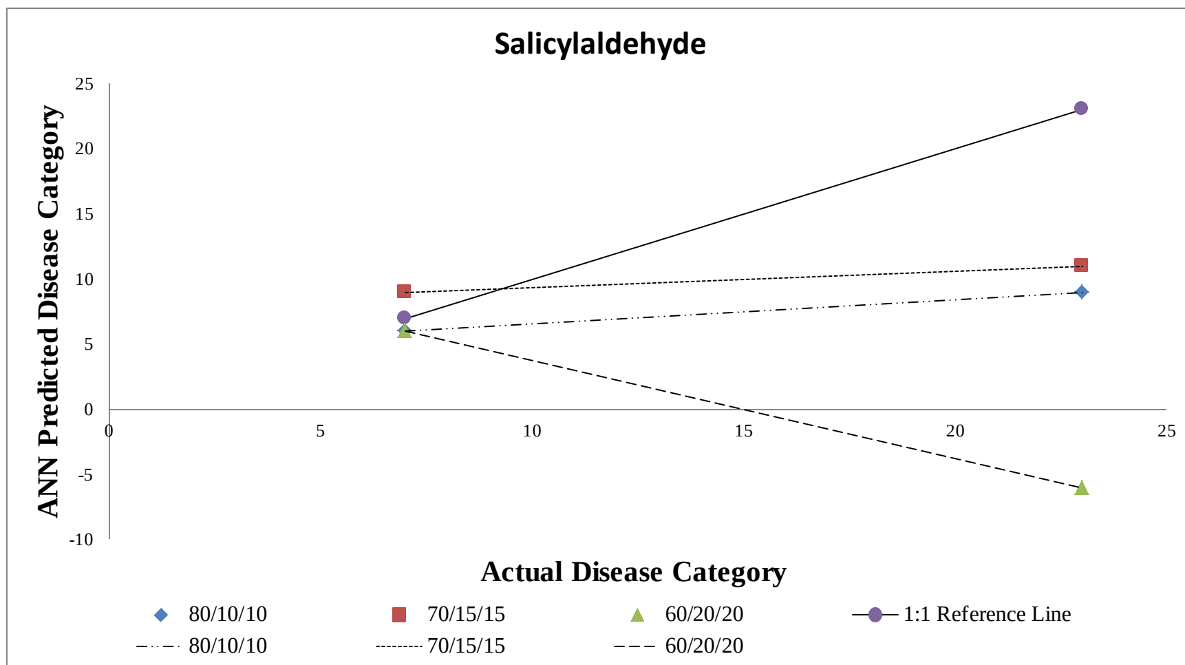
Figure 18: Salicylaldehyde
