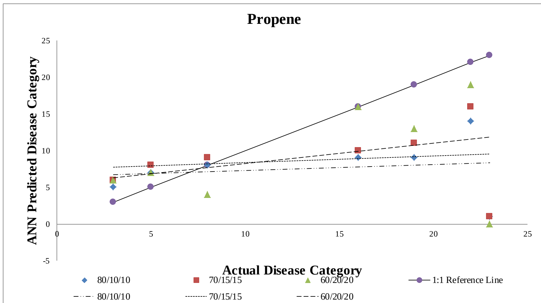
Figure 17: Propene
