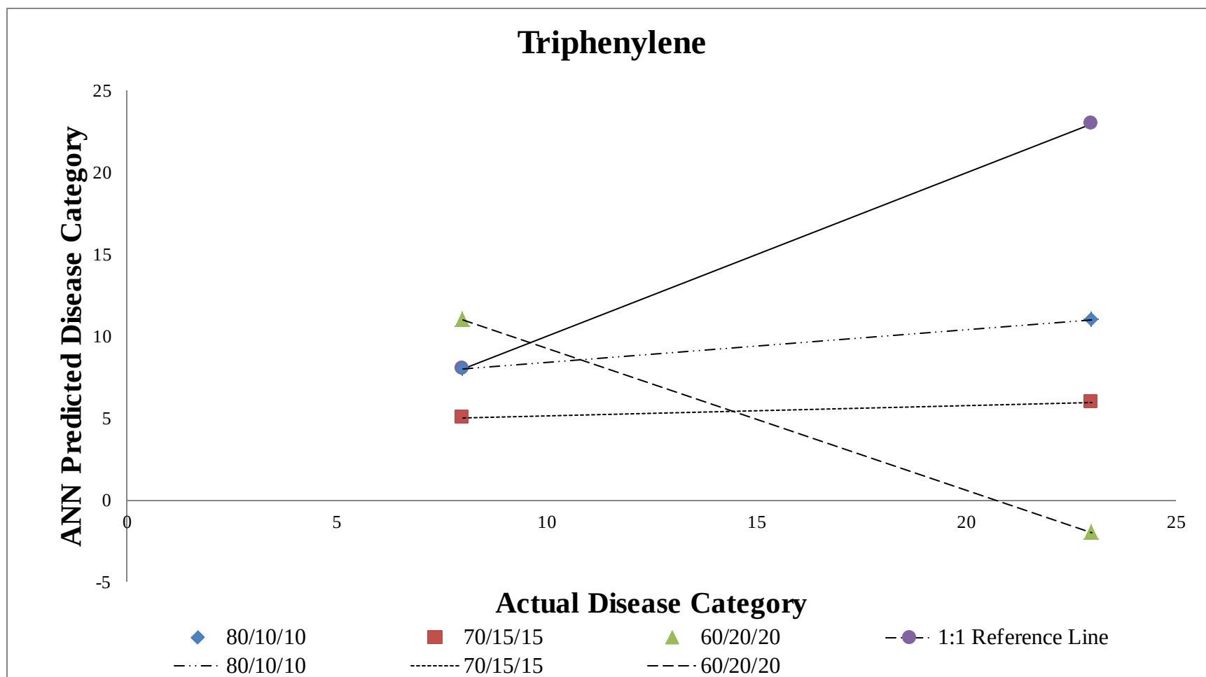
Figure 20: Triphenylene
