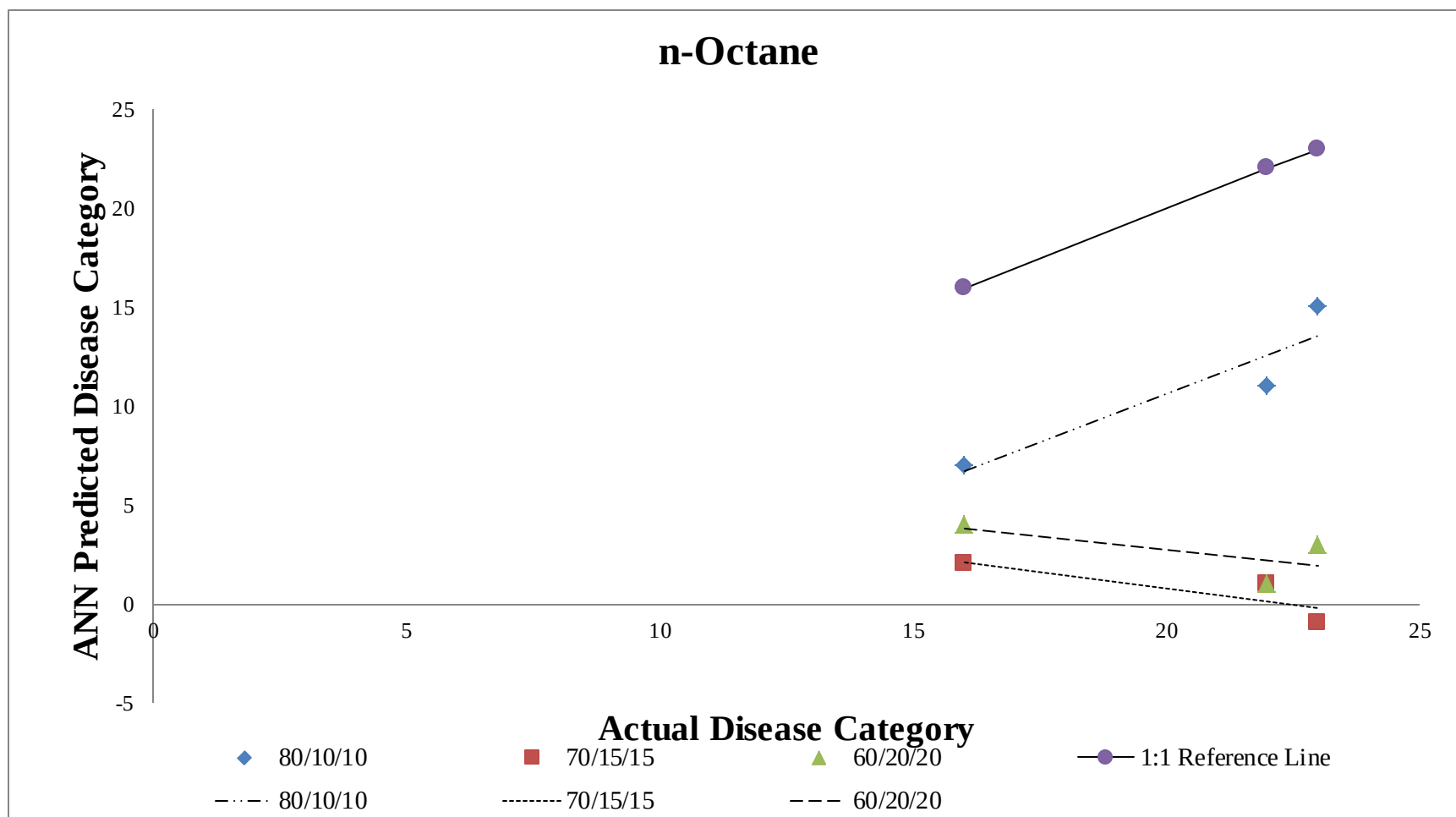
Figure 16: n-Octane
