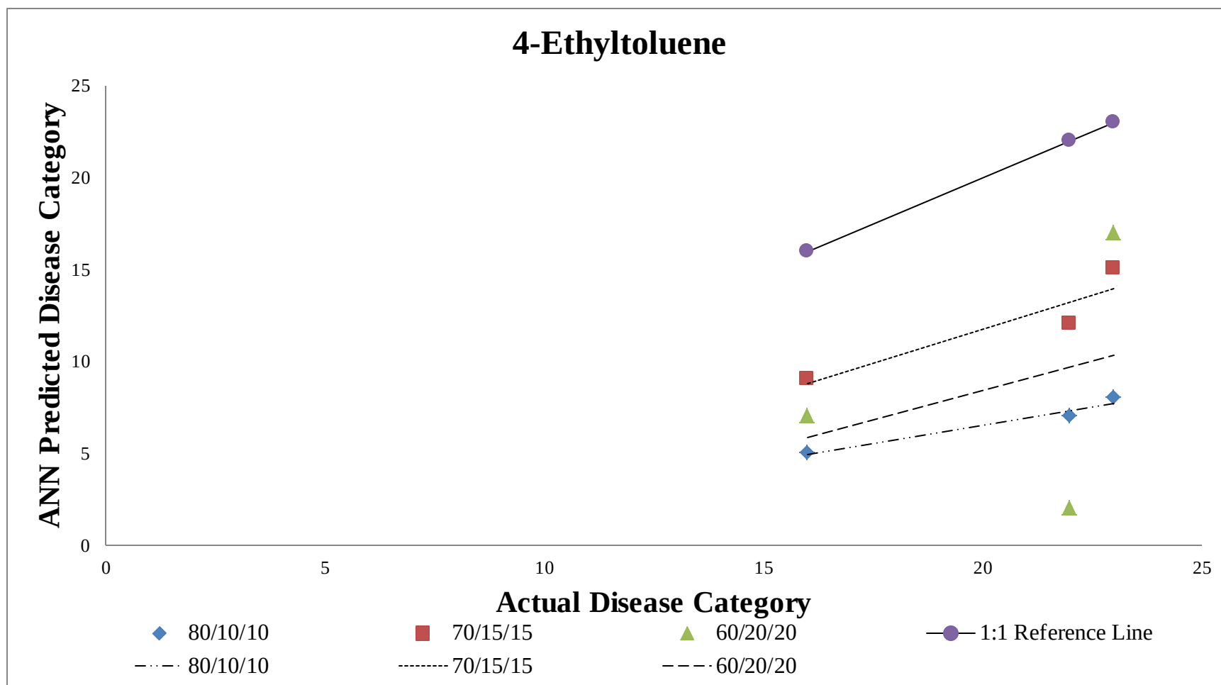
Figure 12: 4-Ethyltoluene
