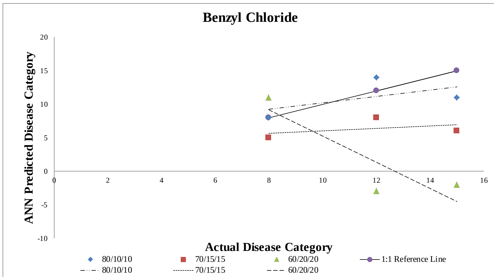
Figure 14: Benzyl Chloride
