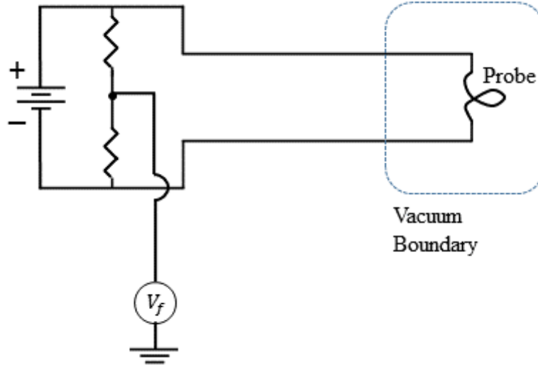
Figure 3.9: Emissive probe circuit diagram.
